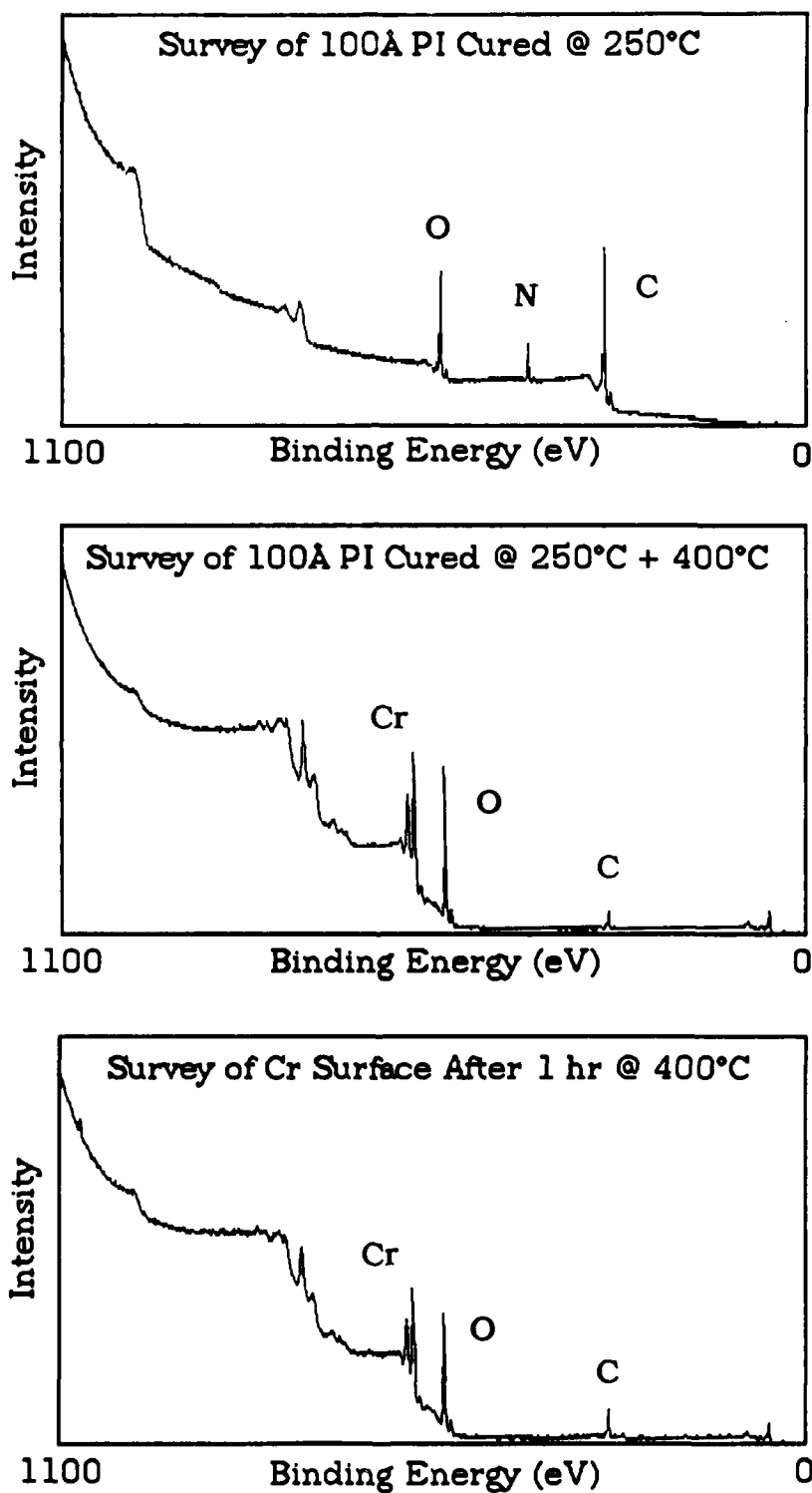
Figure 6-17. XPS Analysis of Cure Temperature Effect on 100 Å PI/Cr Structure
