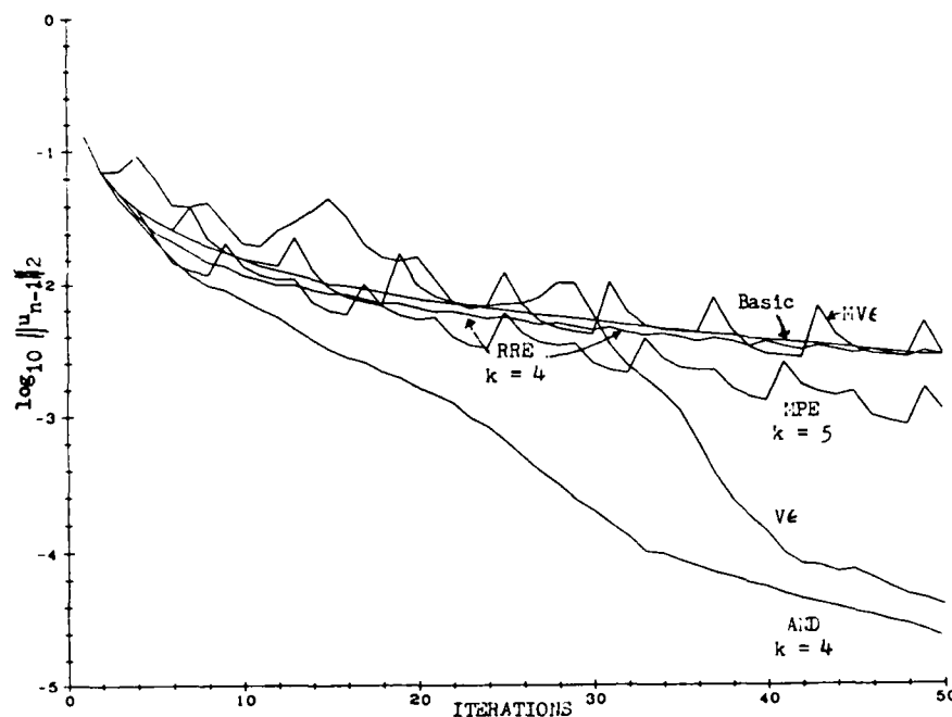
Figure 34. Results for Example 10: AND, MPE, RRE, MV \epsilon , and V \epsilon
