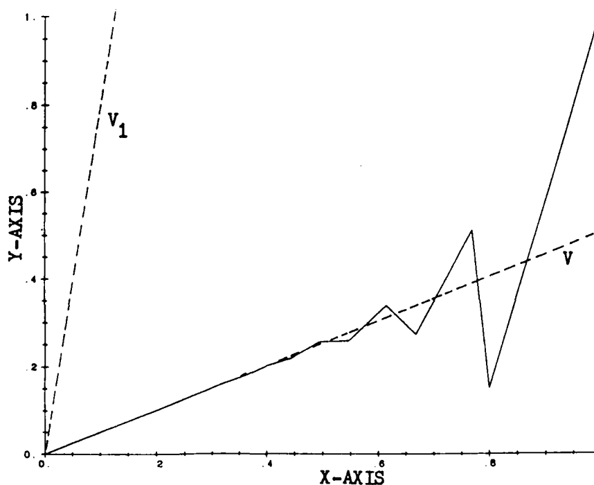
Figure 4. Trajectory for Eigenvalues -0.9 and 0.5
