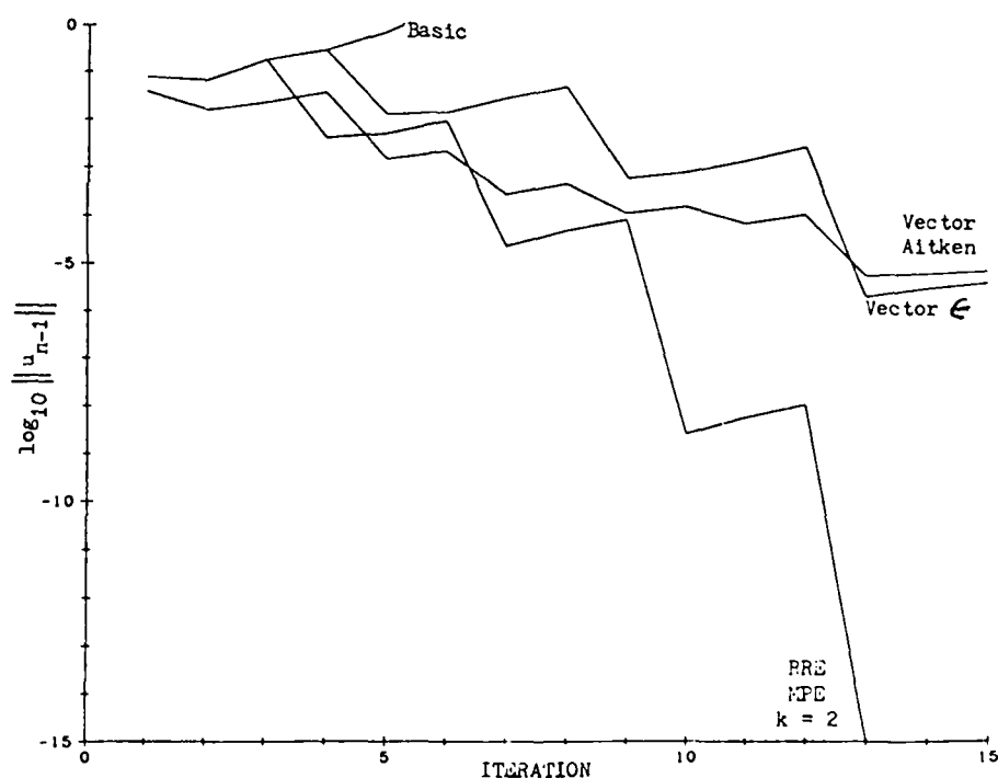
Figure 15. Graph Comparisons for Problem (58)
