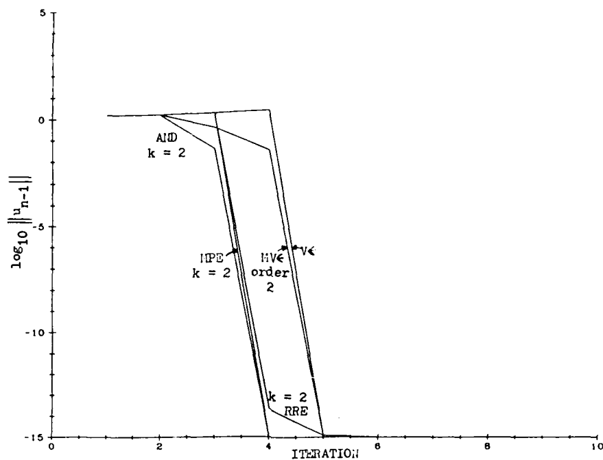
Figure 20. Results for Example 1: AND, MPE, RRE, MV\epsilon , and V\epsilon
