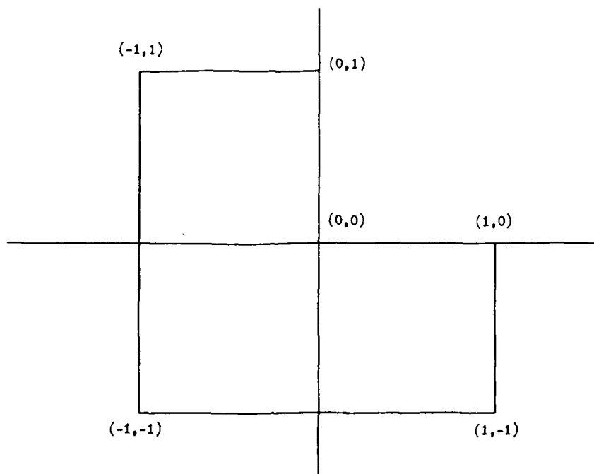
Figure 33. "L" Shaped Region for Example 10
