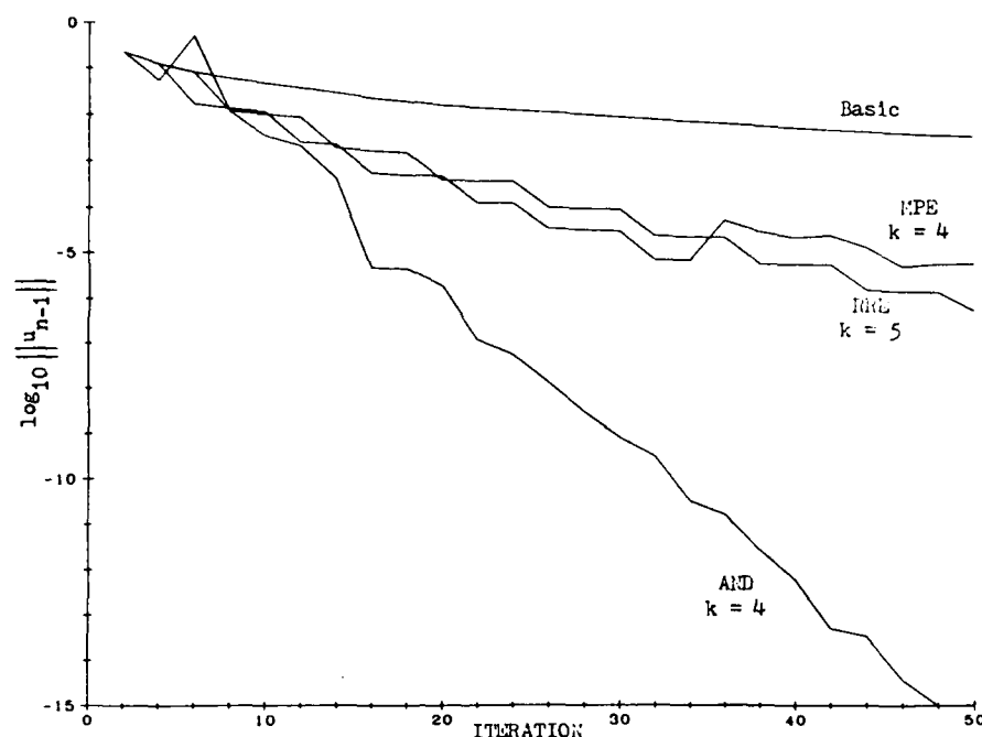
Figure 31. Results for Example 8: Rall's Problem with \pi_0 = 1
