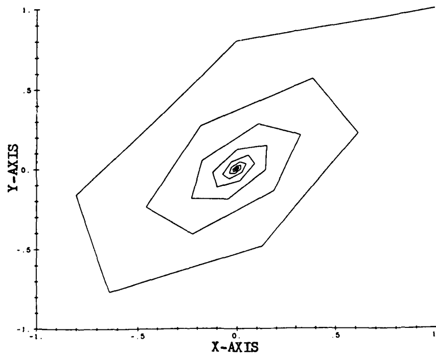
Figure 6. Trajectory for Eigenvalues 0.4 \pm 0.8i
