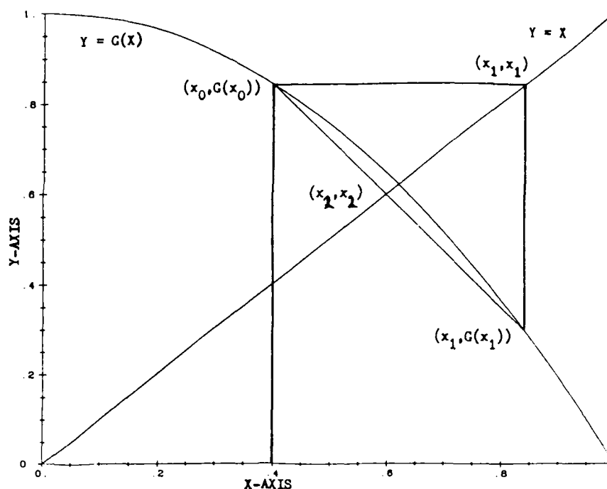
Figure 16. Graph of One Extrapolation of Secant Method
