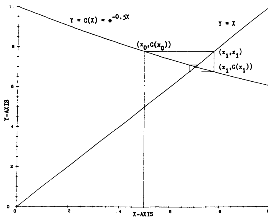
Figure 2. Graphs of y = G(x) = e^{-0.5x} and y = x
