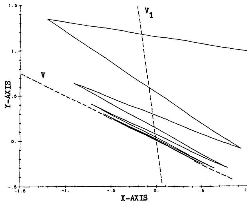
Figure 5. Trajectory for Eigenvalues 0.9 and -0.5
