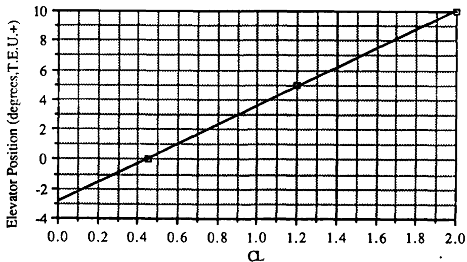
Figure 28. PIONEER (small tail) - Elevator Trim vs CL
