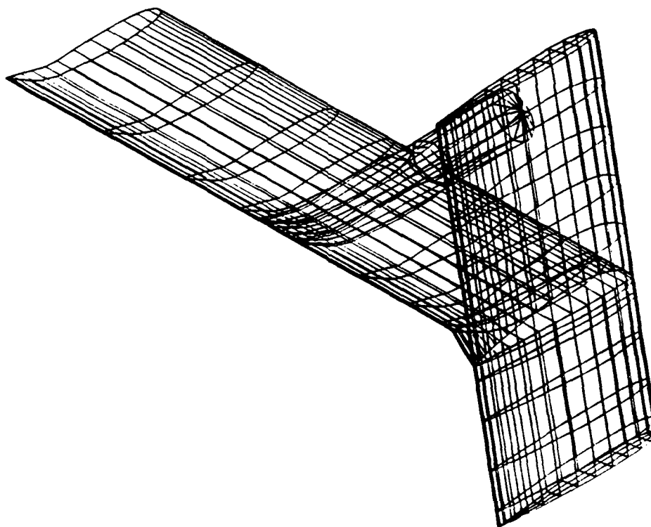
Figure 23. PIONEER Large Tail, 20° Up Elevator
