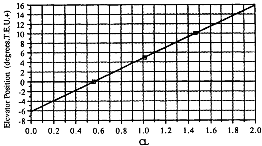
Figure 27. PIONEER (large tail) - Elevator Trim vs CL
