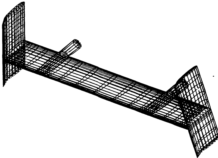
Figure 33. PIONEER Large Tail, 20° Dual Rudder Deflection, 5° Up Elevator
