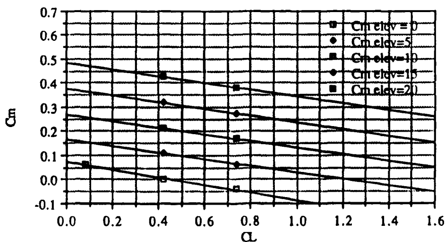
Figure 26. PIONEER (small tail) - C_m vs C_L (T.E.U.+)
