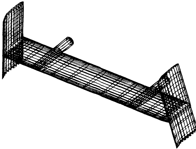
Figure E.13. PIONEER (large tail) - Horizontal Tail/Vertical Tail With 20° Rudder Deflection
