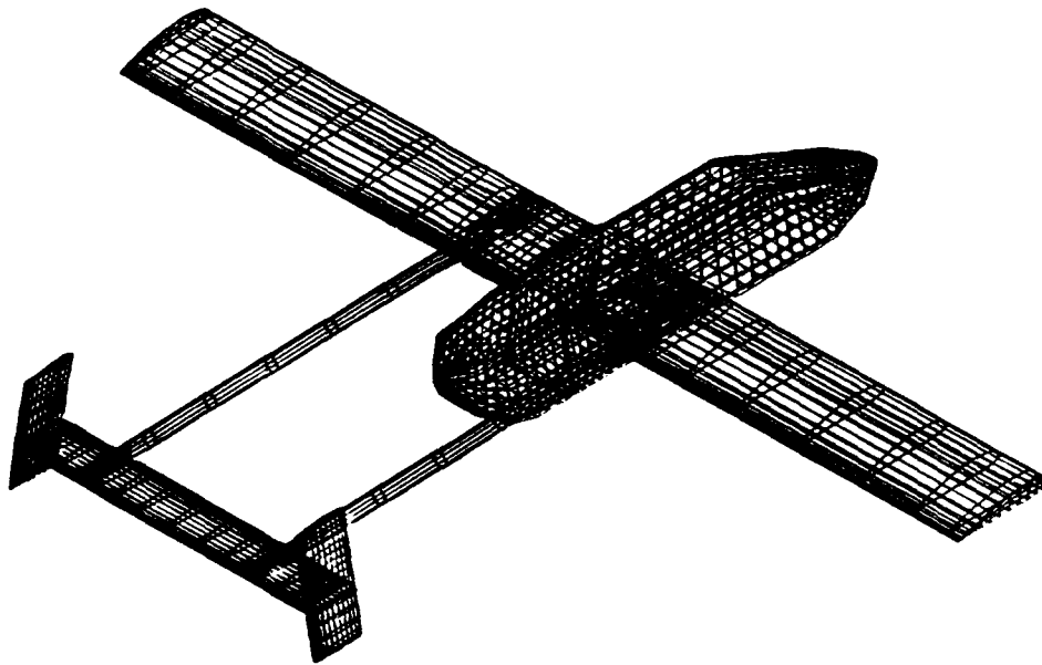
Figure 5. PIONEER (large tail)
