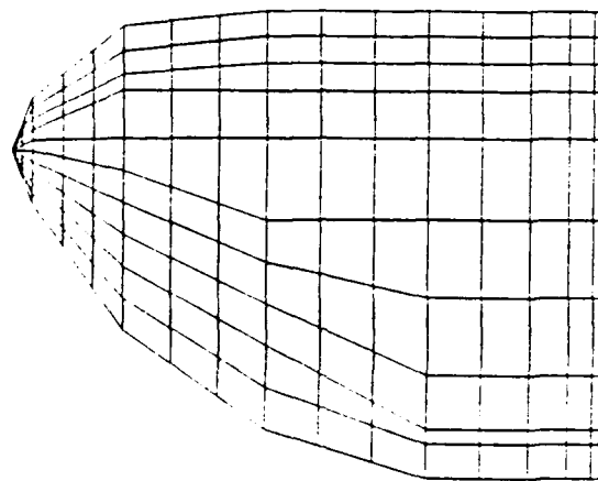
Figure E.6. PIONEER Fuselage Rear
