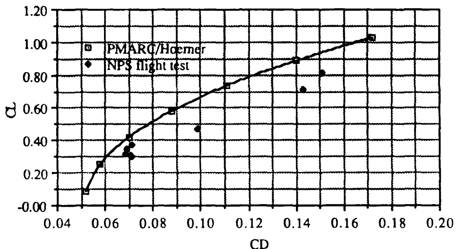
Figure 39. PIONEER (half-scale) - CL vs CD (Total)
