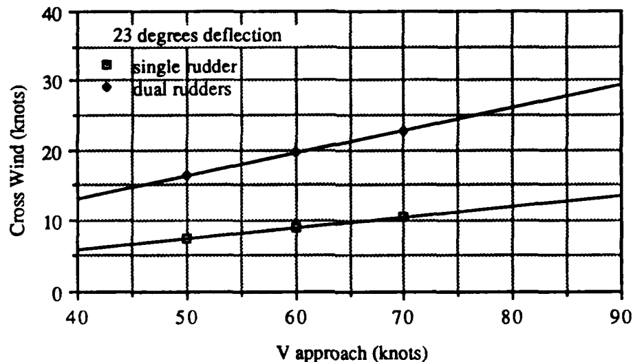
Figure 36. PIONEER - Cross Wind Limit vs Approach Speed
