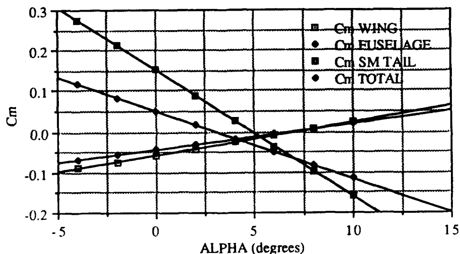
Figure 13. PIONEER (small tail) - C_m vs Alpha
