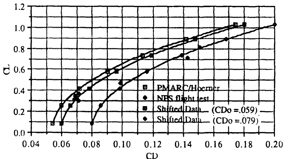
Figure 40. PIONEER (half-scale) - CL vs CD (Total)
