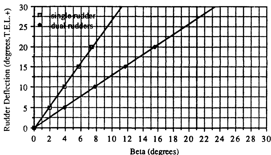
Figure 35. PIONEER - Rudder Trim vs Beta
