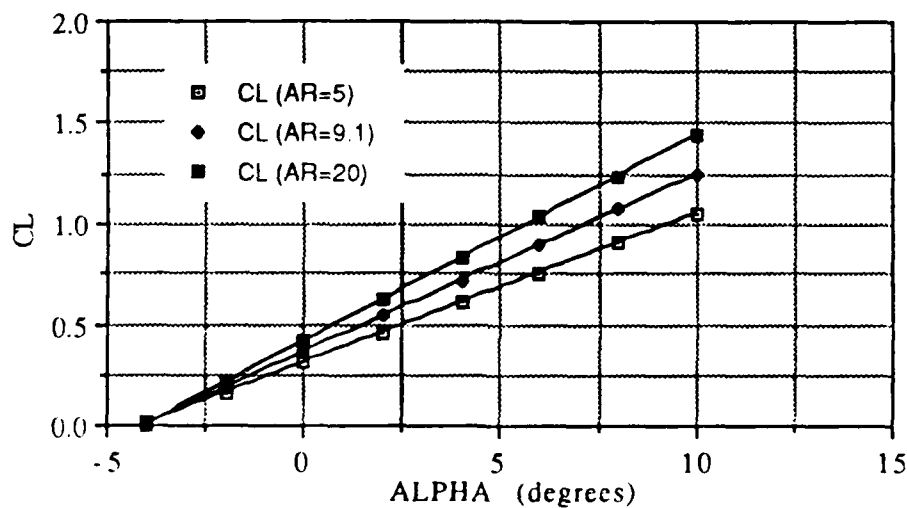
Figure 2. CL vs Alpha (NACA 4415 Wing)
