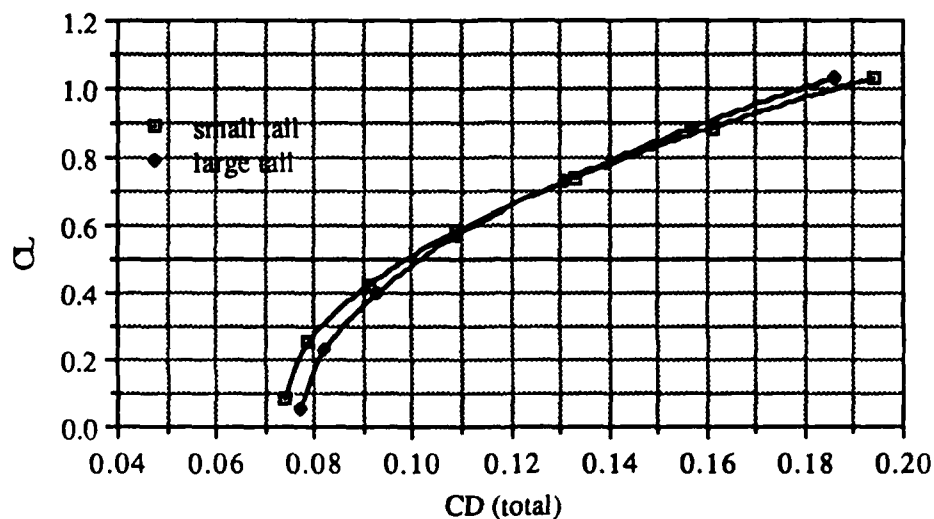
Figure 38. PIONEER - CL vs CD (Total)
