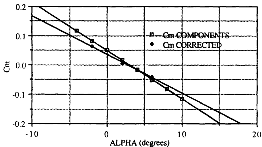
Figure 17. PIONEER (small tail) - C_m vs Alpha
