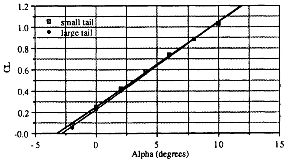
Figure 16. PIONEER (small tail) - CL vs Alpha
