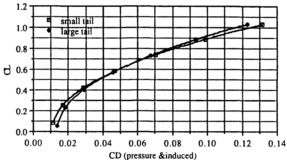
Figure 37. PIONEER - CL vs CD (Pressure and Induced)
