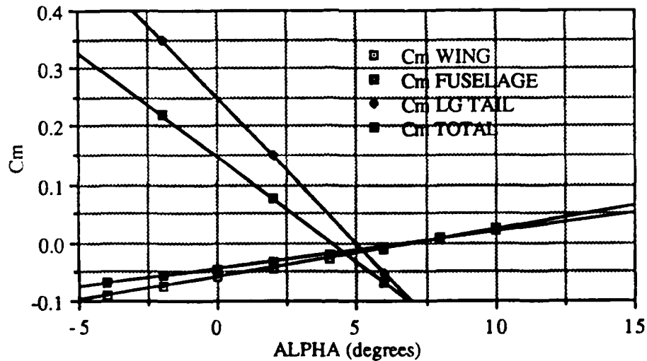
Figure 11. PIONEER (large tail) - Cm vs Alpha
