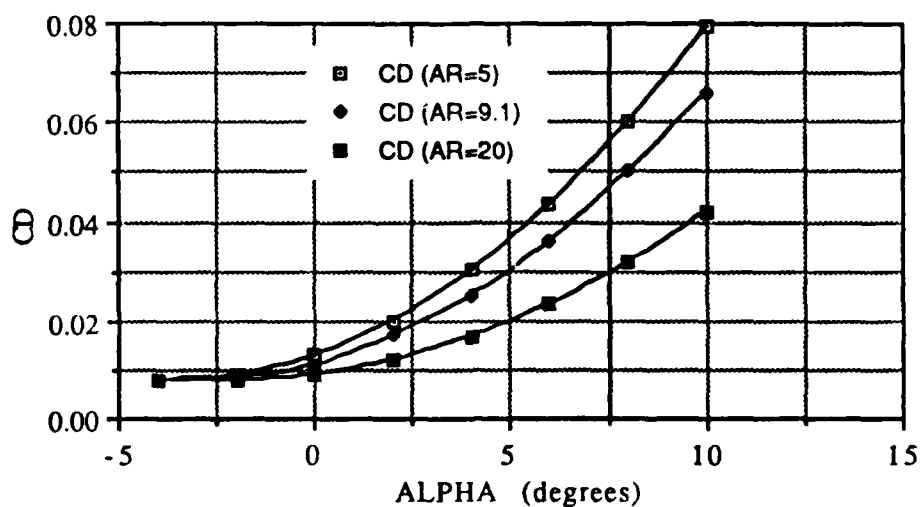
Figure 3. CD vs Alpha (NACA 4415 Wing)
