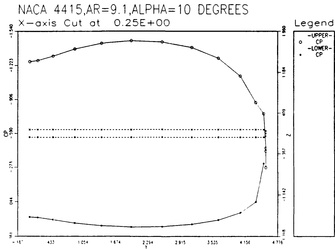
Figure 1.2 Cp vs Y (Span Length)
