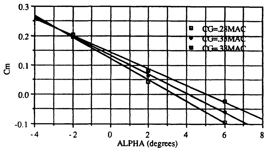
Figure 19. PIONEER (large tail) - Cm vs Alpha
