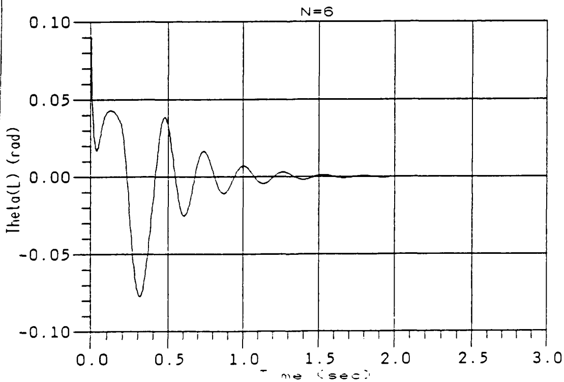
Figure 6.11: Appendage Deformation at Secondary Mirror for 30deg. Slew
