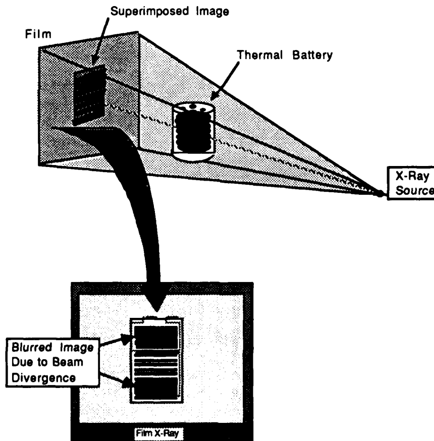
Figure B1-1 Shadowgraph image from film radiography
