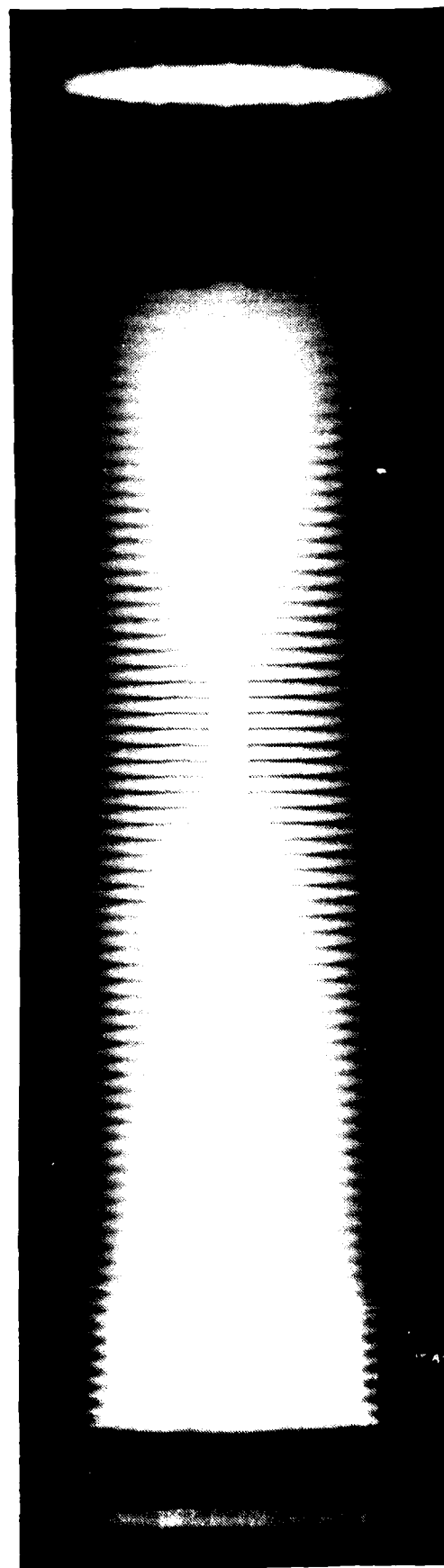
Figure 3.1-17 Film radiograph of battery #106
