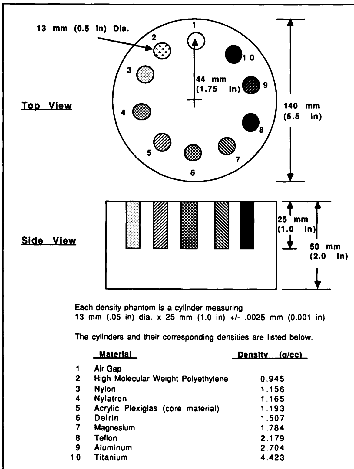
Figure A3-1 Density calibration standard
