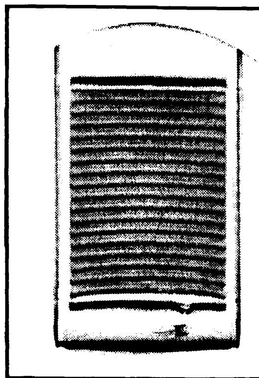
Figure 3.1-35 CT view of spent squib in battery #112
