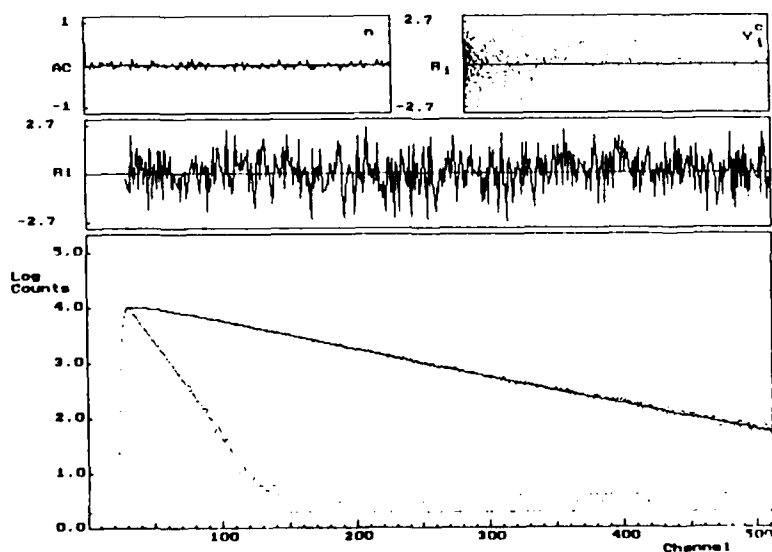
Figure 6 : Decay curve of the fluorescence of P3N ( 6 \cdot 10^{-6}M ) adsorbed on Ludox WP 0.1 % , with ( 1.2 \cdot 10^{-6}M ) CTAC exc. = 330nm, em. = 487nm.
