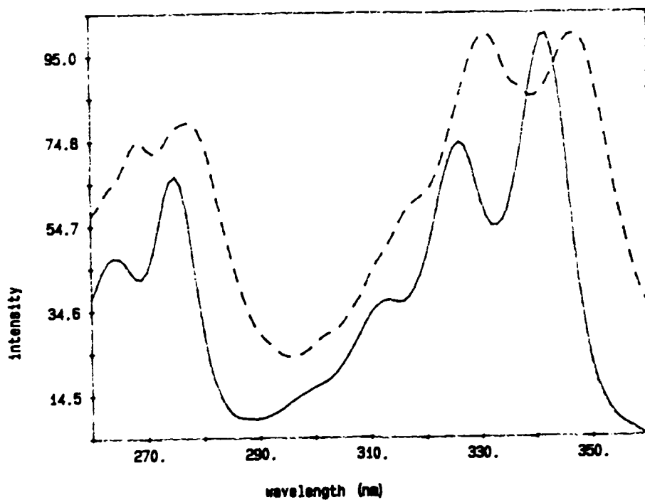
Figure 2 : Excitation spectra of ( 6 \times 10^{-6} \text{ M} ) P3N adsorbed on Ludox WP 0.1% (--) I_{em}=378\text{nm} , (....) I_{em}=500\text{nm} .
