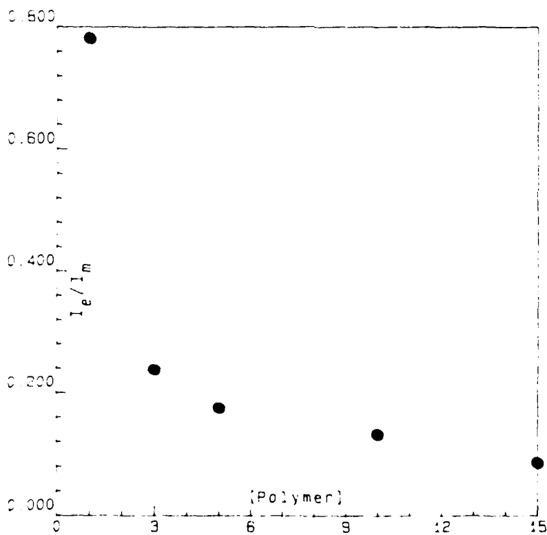
Figure 16 : Variation of the ratio I_E/I_M of P3N as a function of polymer added
