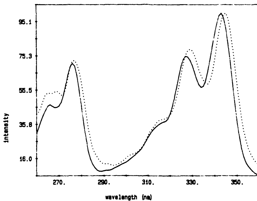
Figure 3 : Excitation spectra of ( 6 \times 10^{-6} \text{ M} ) P3N adsorbed on Ludox WP 0.1% with 5 \times 10^{-5} \text{ M} CTAC (--) I_{em}=378\text{nm} , (....) I_{em}=500\text{nm} .
