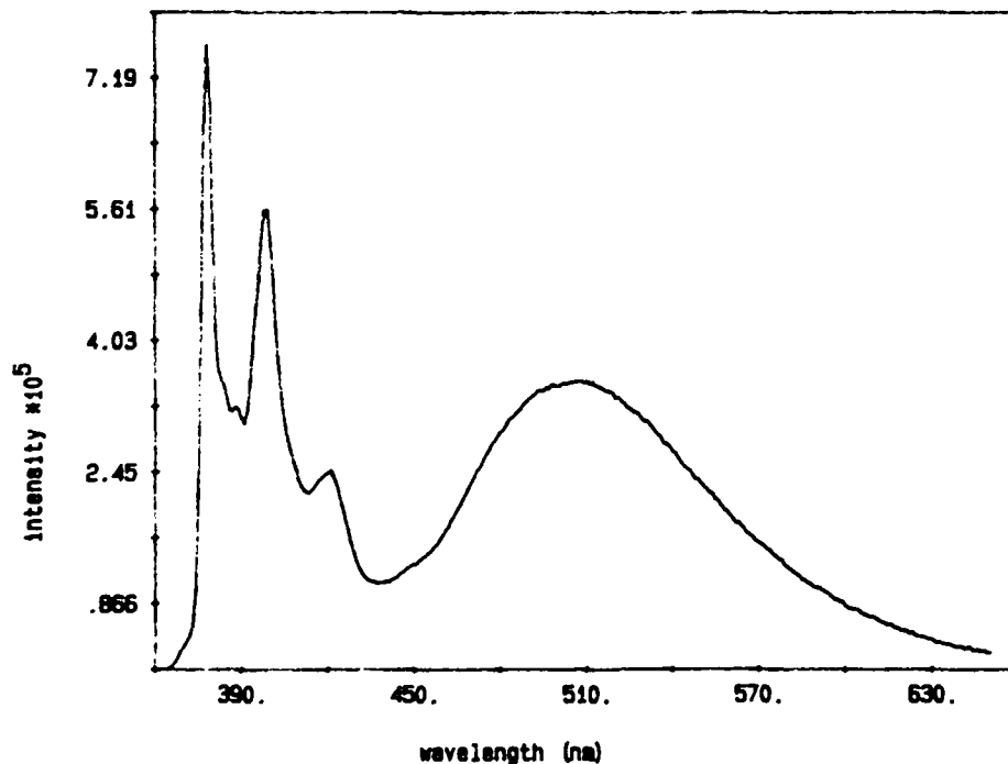
Figure 1 : Emission spectrum of ( 6 \cdot 10^{-6} M) P3N adsorbed on Ludox WP 0.1 %
