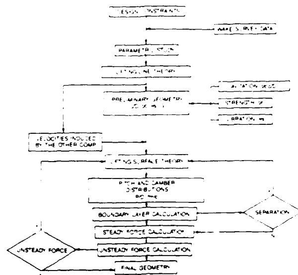
Fig. 1. Flow chart of CR propeller design methodology.
