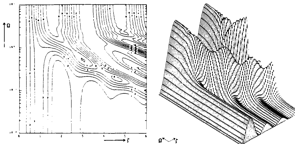
Figure 3 Sinusoidal grating. +1 diffraction efficiency, for m = +1 on-Bragg replay, as a function of the modulation parameter \xi and the volume parameter \Omega . Note the logarithmic \Omega scale. In the contour plot, contour 1 = 10% efficiency, 2 = 20% etc.
