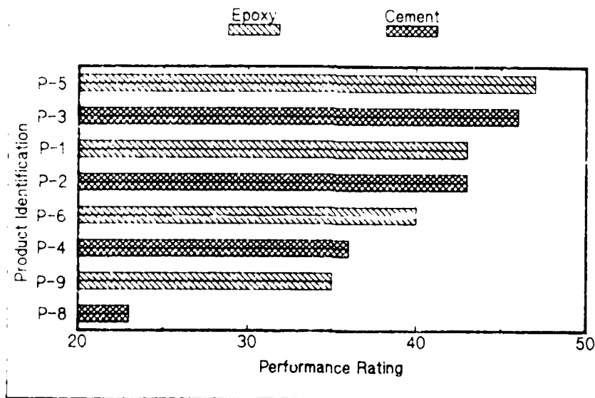
Figure 17. Overall performance ratings for individual repair materials
