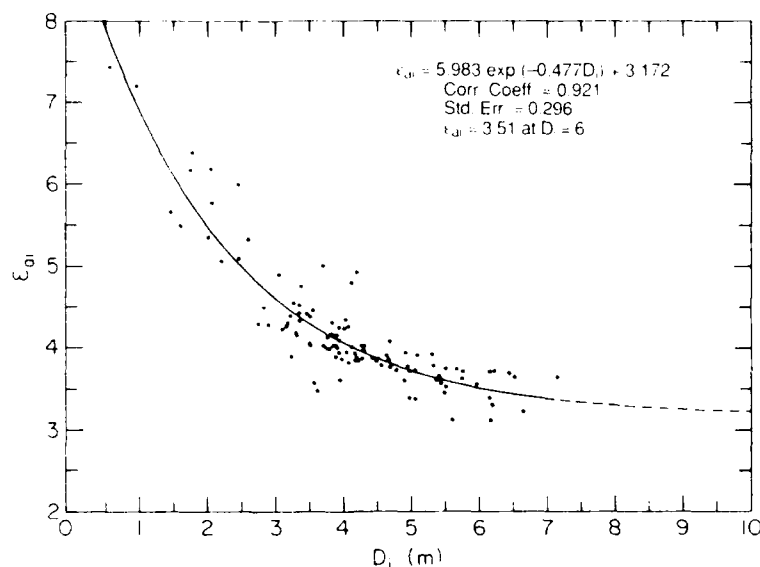
Figure 7. Relative apparent dielectric constant for ice, E_{ai} , vs ice thickness, D_i , for 1987 data obtained with the 120-MHz antenna.
