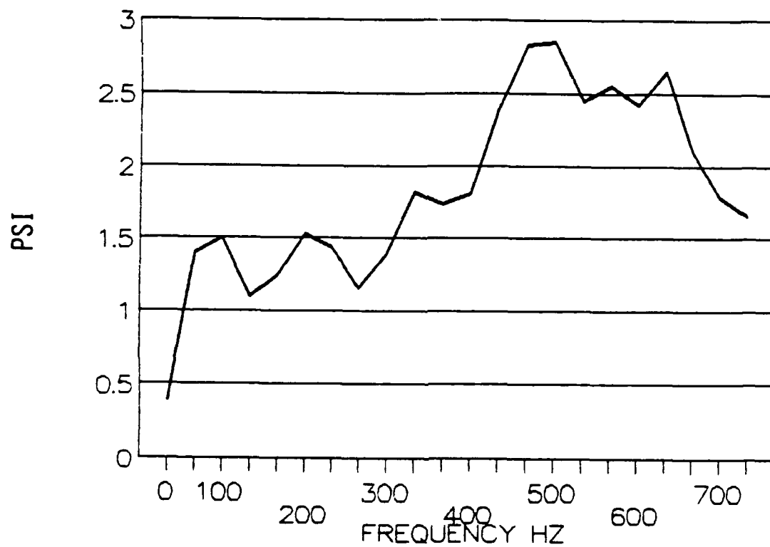
Figure 5-6, Pressure Into Chopper VS Frequency
