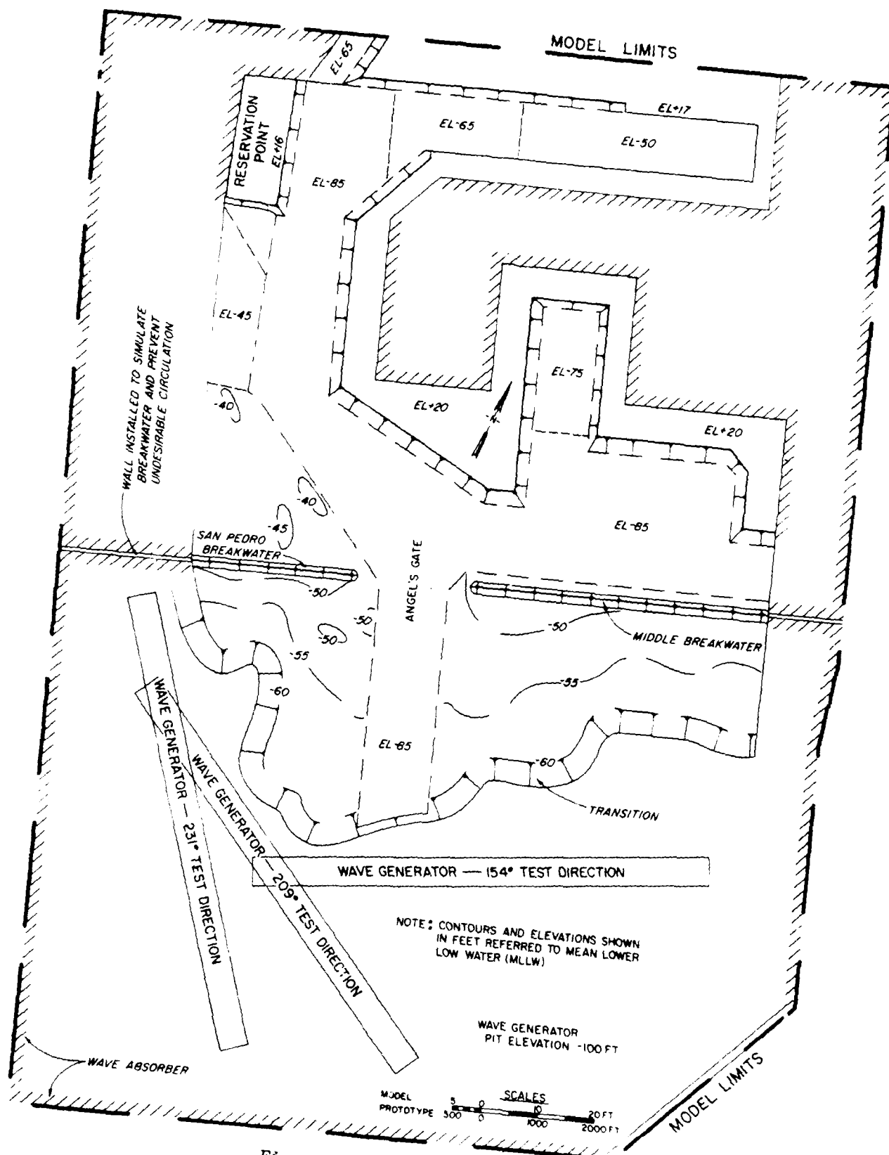
Figure 4. Model layout
