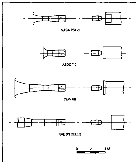
Fig. 4-2 Comparison of inlet and exhaust geometries — altitude cells
