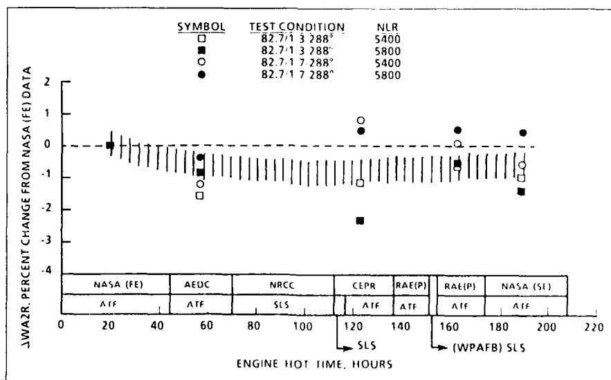
Fig.11-2 Engine airflow change as a function of engine operating time
