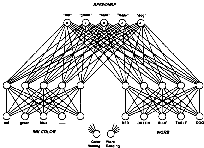
Figure 10. The network used to simulate response set effects and the dilution effect. The numbers that appear with each output unit are the bias terms that were assigned to these units during testing (see text for an explanation).
