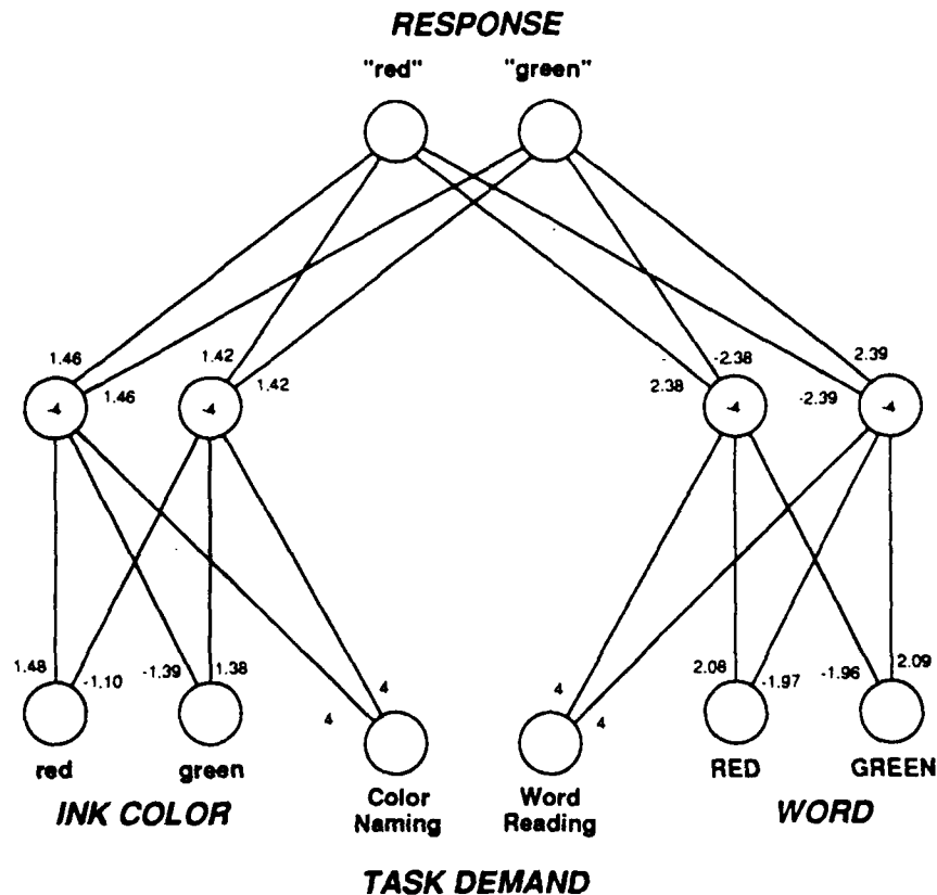
Figure 4. Diagram of the network showing the value of the weights after training on the word reading and color naming tasks.
