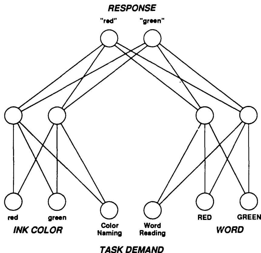
Figure 2. Network architecture. Units at the bottom are input units, and units at the top are the output (response) units.
