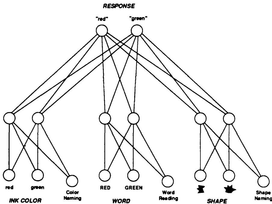
Figure 8. The network architecture used to simulate the shape naming experiments conducted by MacLeod and Dunbar (1988).
