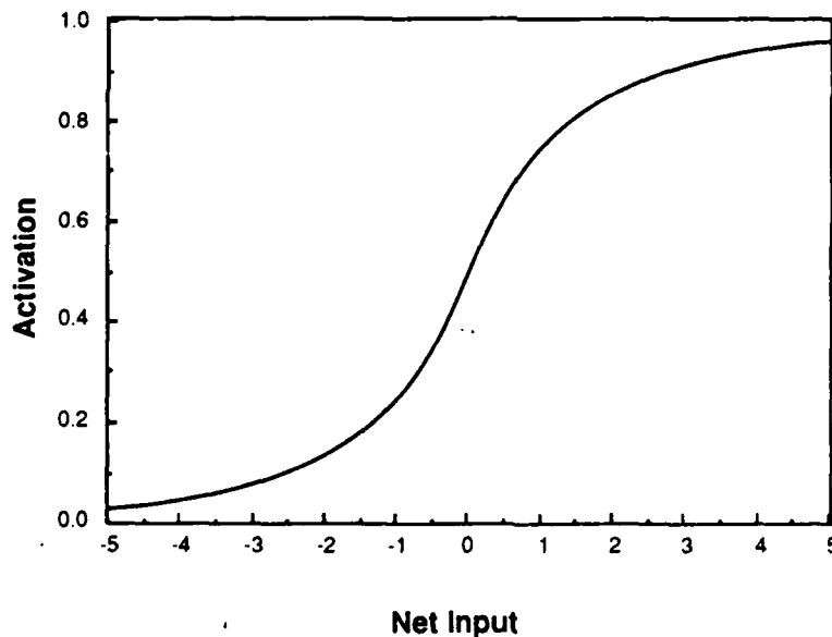
Figure 3. The logistic function. Note that the slope of this function is greatest when the net input is 0.0, and decreases when the net input is large in either the positive or negative directions.
