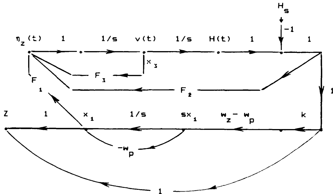
Figure II.5 Signal Flow Graph of the Controller
