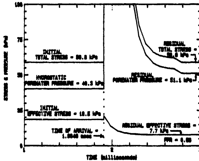
Figure 8.24b Magnified record.
