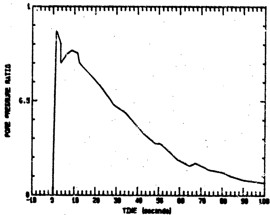
Figure 8.13 Porewater pressure dissipation - 0.25 kg charge.
