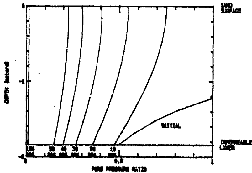
Figure 8.27 Dissipation of excess porewater pressure versus depth - analytical model simulation, Test S1.
