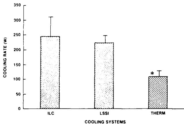
Fig. 1. Calculated cooling rates ( \bar{X} , S.D.) provided by the three microclimate systems.
