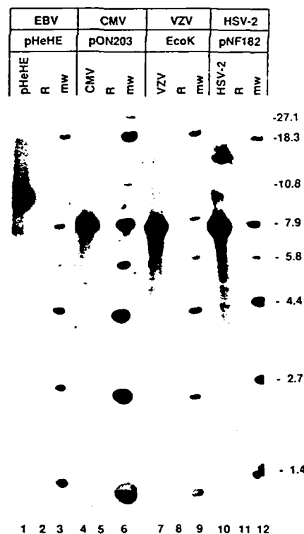
FIG. 6. Hybridization tests using probes derived from other herpesviruses. The blot contained DNA from HHV-7 (RK)-infected cells (lanes 2, 5, 8, and 11), pHeHE DNA (lane 1, Bam HI-digested), HCMV (Towne)-infected cell DNA (lane 4, Bam HI-digested), VZV DNA (lane 7, Eco RI-digested), and DNA from HSV-2-infected cells (lane 10, Bgl II-digested). The probes contained 2-kb EBV DNA (pHeHE), 7.6-kb HCMV DNA (pON203), 7.3-kb VZV DNA ( Eco K), and 7.6-kb HSV-2 DNA (pNF182) fragments. mw, Size markers.
