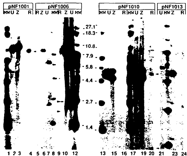
FIG. 5. Hybridizations using HHV-6 (Z29) probes. Blots containing Hind III digests of DNAs from cells infected with HHV-6 [Z29 (Z) or U1102 (U)] or with RK isolate 2 (R) were hybridized with the HHV-6 (Z29) probes shown. Lanes 9–12 show long exposure of lanes 5–8, and lanes 17–20 show long exposure of lanes 13–16. The HHV-7 (RK) hybridized bands are marked with arrowheads. MW, size markers.
