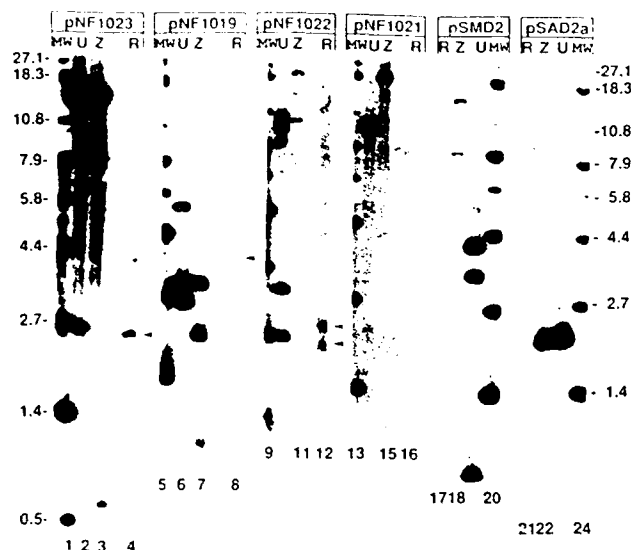
FIG. 4. Hybridization of HHV-6 (U1102) probes to HHV-6 [Z29 (Z) or U1102 (U)] and to RK virus isolate 2 (R) DNAs. Hind III-digested DNA was blotted and hybridized with the 32 P-labeled probes shown. MW, size markers that hybridize with the plasmid portions of the probes. Arrowheads point to the hybridizing HHV-7 (RK) bands.
