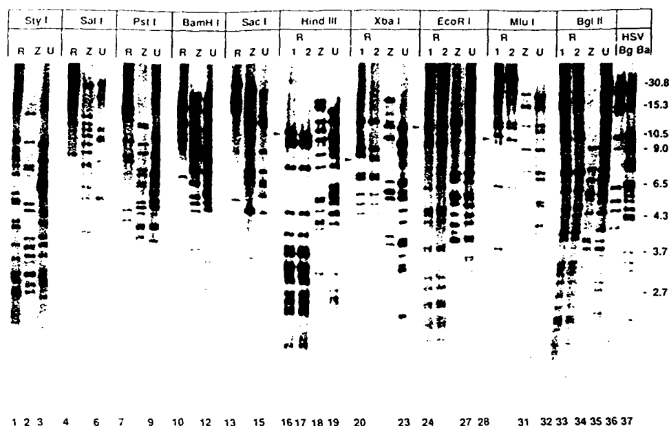
FIG. 2. Restriction enzyme patterns. ^{32} P-labeled DNA was prepared from PBL cultures infected with HHV-6 strain U1102 (U) or Z29 (Z) or with HHV-7 strain RK (R). Cleavage of DNA from isolates 1 and 2 with Hind III, Xba I, Eco RI, and Mlu I produced similar patterns except the variant bands marked with arrowheads. The Bgl II patterns exemplify patterns in which no differences can be detected in the migration of fragments of isolates 1 and 2. In the Sty I, Sal I, Pst I, Bam HI, and Sac I patterns, no differences are noted and hence only isolate 2 is shown. The lack of variations with some enzymes probably reflects variable bands that comigrate with other bands in the gel. Lanes 36 and 37 contain size markers consisting of Bgl II (Bg)- or Bam HI (Ba)-cleaved ^{32} P-labeled DNA from Vero cells infected with HSV-1 (Justin). Marker sizes are indicated in kilobases (kb) at right.
