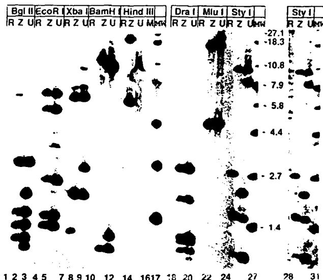
FIG. 3. Hybridization of pHD9 to infected-cell DNAs. Lanes 1–27: hybridization with ^{32} P-labeled pHD9 probe derived by Honess and coworkers from HHV-6 (U1102). The blot contained restriction enzyme-cleaved DNAs from mock-infected cells (M) or from cells infected with HHV-6 strain Z29 (Z) or U1102 (U) or with RK virus (R). The blot was then hybridized (without stripping the pHD9 probe) with ^{32} P-labeled RK virus DNA labeled in vivo . Lanes 28–31: rehybridized blot portion shown in lanes 24–27. Lanes 17, 27, and 31: molecular weight (mw) markers that hybridize with the plasmid portion of the pHD9 probe; sizes are indicated in kilobases.
