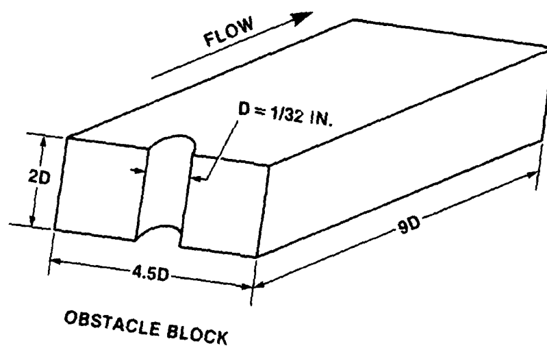
Fig. 4. Obstacle block.
