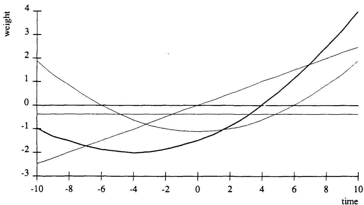
Figure 5-5: A graph of the inputs to a unit regarded as a convolution function and decomposed into constant, even, and odd components.
