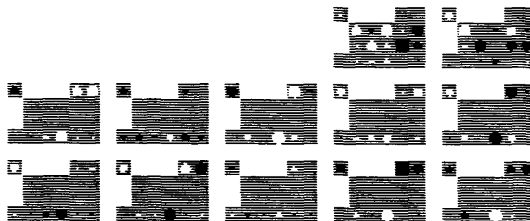
Figure 5-9: This network was trained on 298 samples taken uniformly from the phase space of a simulated arm. The inputs (from left to right) are the position, velocity and desired acceleration of the shoulder joint and the position, velocity and desired acceleration of the elbow joint. The magnitude of the largest weight is 9.63.
