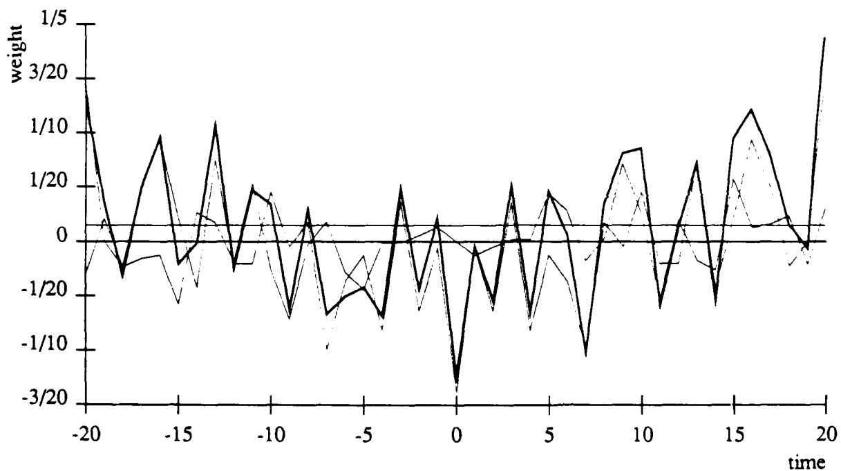
Figure 5-7: A graph of the inputs to a unit regarded as a convolution function and decomposed into constant, even, and odd components.
