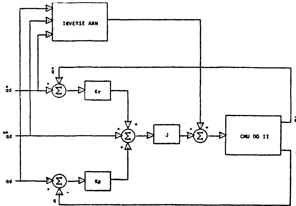
Figure 2-1: Block diagram of a feedforward torque controller, taken from [Khosla 86, page 114].
