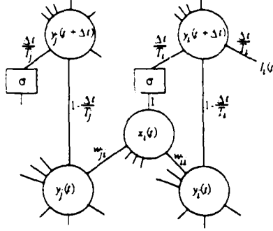
Figure 2: A lattice representation of (4).
