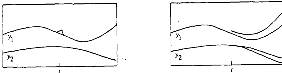
Figure 1: The infinitesimal changes to y considered in e_1(t) (left) and z_1(t) (right).
