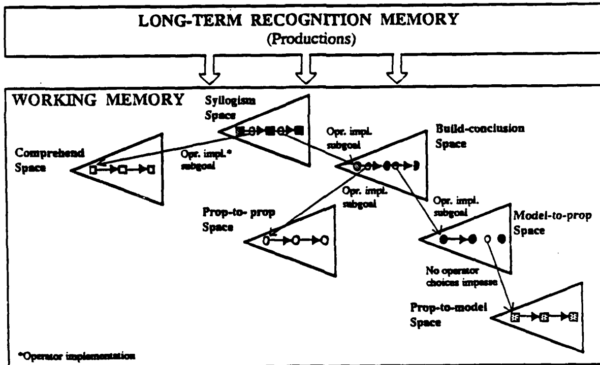
Figure 2: The structure of Soar.
