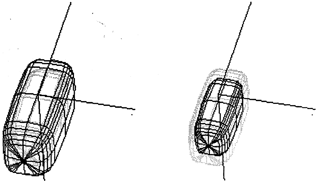
Figure 5.1: \beta expansion and contraction of a superquadric model. left : \beta = 1.2 , right = \beta = 0.8 .
