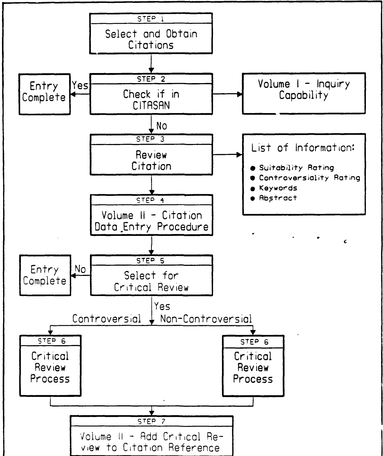
FIGURE 1. BLOCK DIAGRAM OF THE GENERAL PROCESS FOR ADDING NEW CITATIONS TO CITASAN
