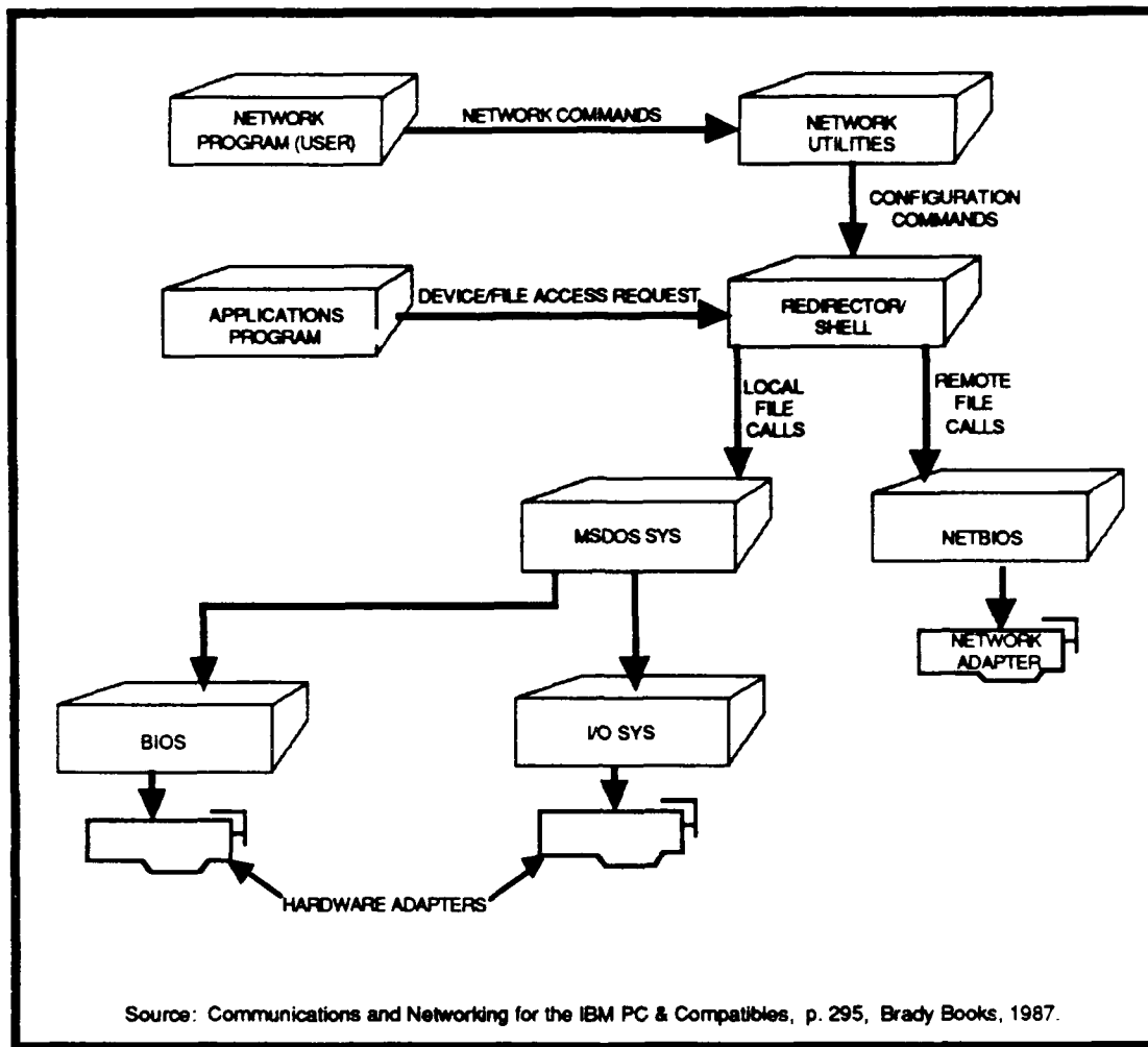
Figure 6. LAN Software Relationships
