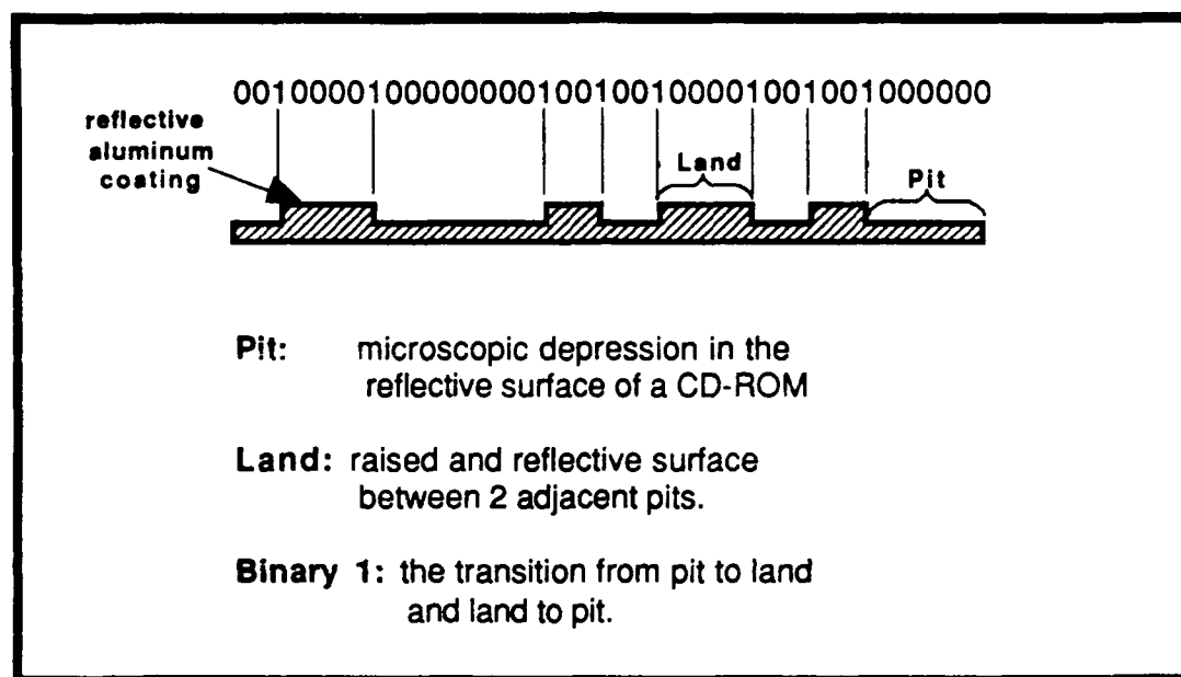
Figure 11. Physical Construction of CD-ROM
