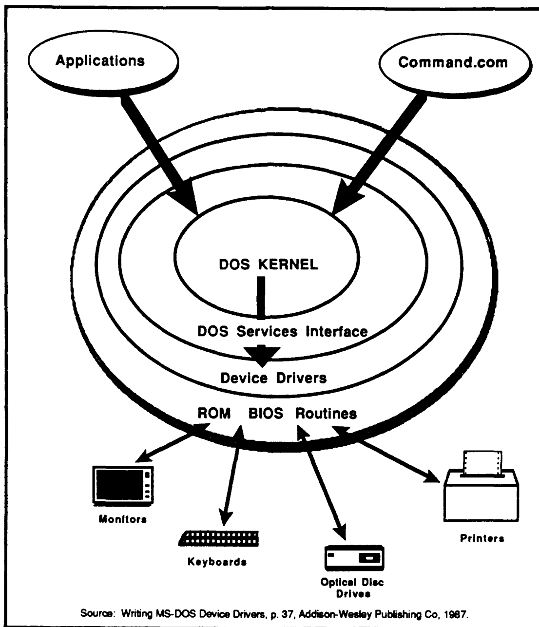
Figure 4. MS-DOS/ROM-BIOS Interface
