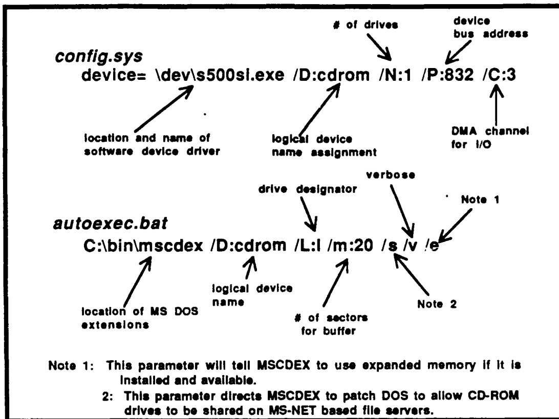
Figure 16. MS-DOS CD-ROM Extensions Installation
