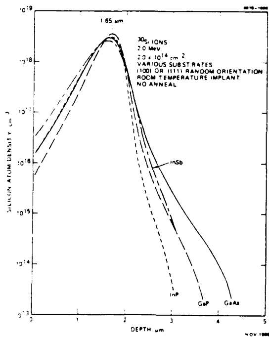
Fig. 27. Depth profiles of MeV Si in GaAs, GaP, InP, and InSb
