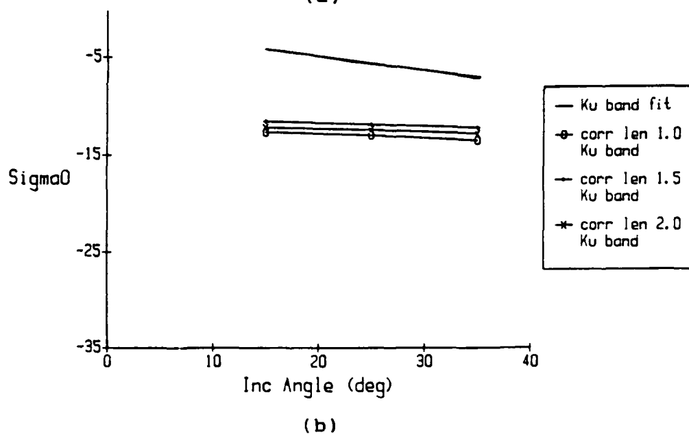
Figure 6.21: Backscatter cross-section of desalinated ice at (a) C band and (b) Ku band, as determined from data obtained during the CRREL'89 experiment, compared with predictions of the Effective Medium theory for three different values of correlation length of spacing between air bubbles.
