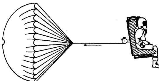
Fig 7 Passive stabilisation by bridle mounting of drogue
