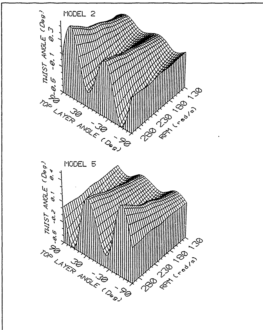
Figure 27 Models 2 and 5 static behavior comparison, inputs are RPM and Laminate Principal Orientation (LPO) angle, output is Tip Twist Angle (TTA).
