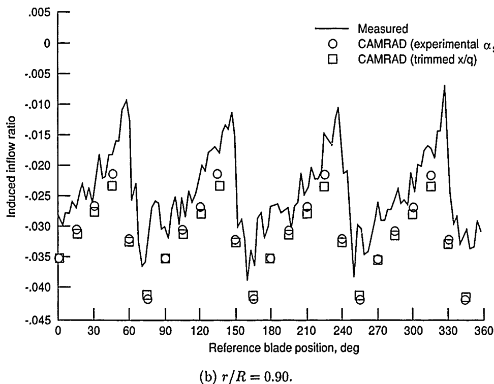
Figure 12. Time history of measured and CAMRAD predicted induced-inflow ratio at \mu = 0.23 and 330^\circ azimuth.
