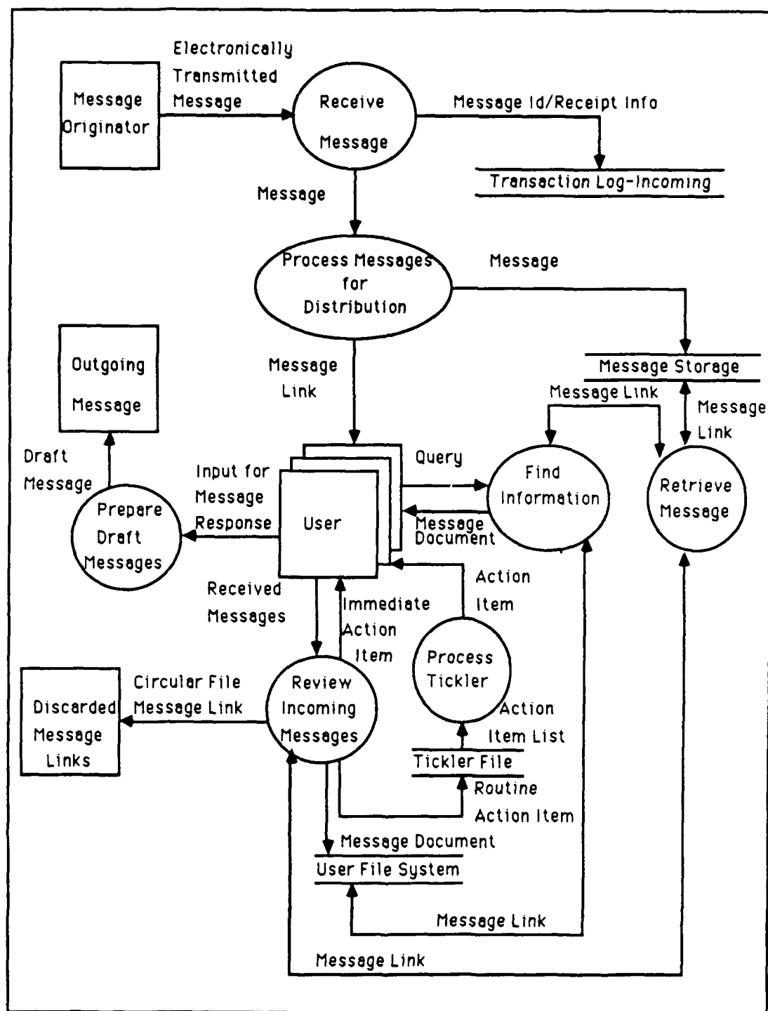
Figure 10. A Model for the Management and Use of Naval Messages
