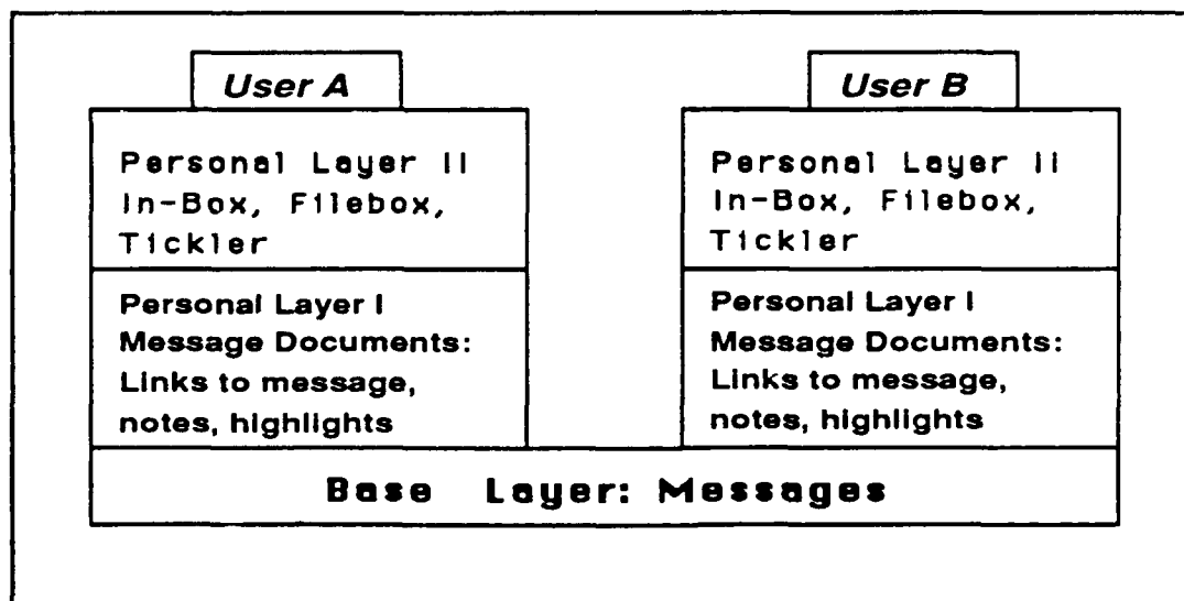
Figure 16. Two Levels of Private Context
