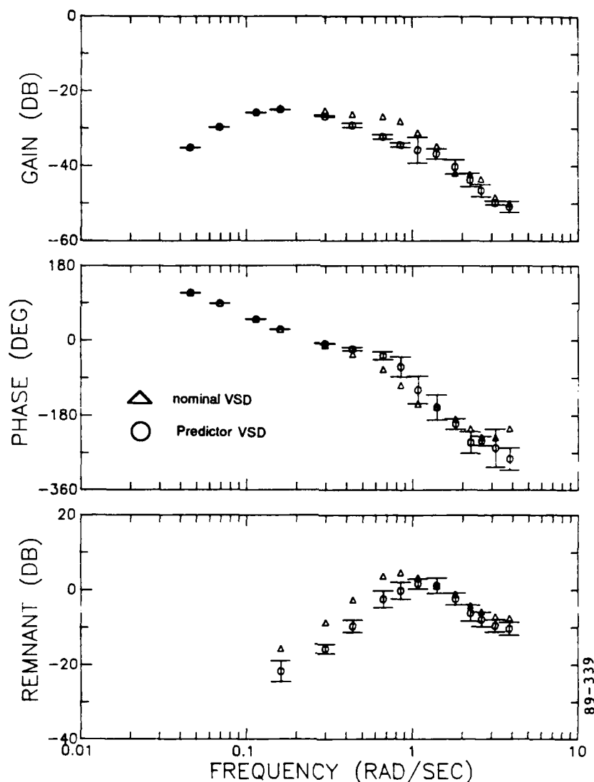
Figure 3.13. Stick Spectrum for Nominal VSD and Predictor VSD
