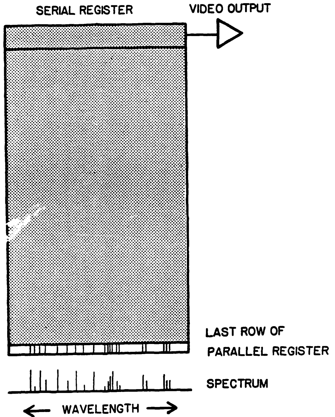
Figure 11 Diagram of CCD used in a Spectral Framing Mode of operation for time resolved spectroscopy.
