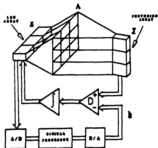
Fig. 3 The Bimodal Optical Computer
