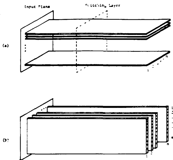
Fig. 2. (a) Stack of m planar arrays of n horizontal channels each. (b) Stack of n planar arrays of m vertical channels each.
