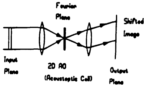
Fig 4. The 2D AO cell shifts the image in any direction by changing the direction of light in the Fourier plane.
