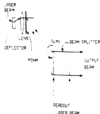
Fig. 4. Page selection and readout. The deflector addresses a single hologram on the POHM and a page of data is written in parallel onto the output laser beam.
