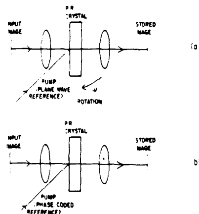
Fig. 6. Photorefractive memory: (a) multiple holograms stored and retrieved as a function of crystal angular positions and multiple holograms are stored and retrieved as a function of phase-coded reference beams.
