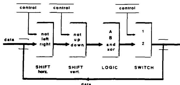
Fig. 11. Functionally programmable module.
