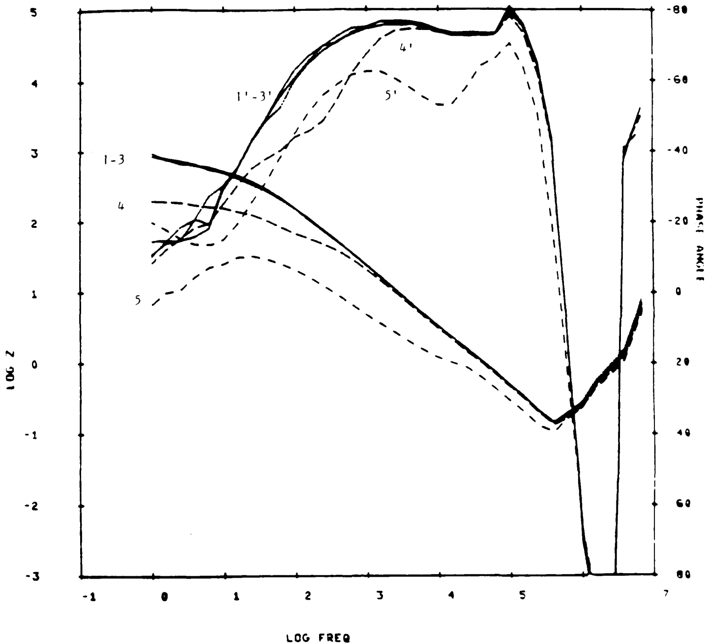
Fig. 11 Impedance and phase angle plots of an 10 cm long Pb strip-line cell in 15 % H_2SO_4 . The curves 1') to 5') .8V to 1.2V. (increment: .1V).
