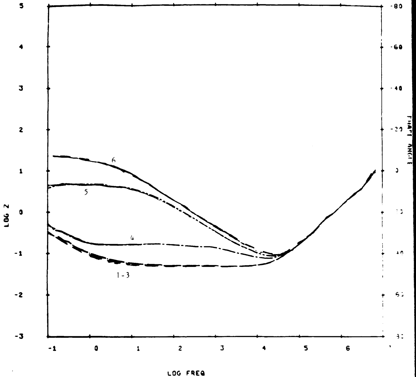
Fig. 12 Impedance plots of an 100 cm long Pb strip-line cell in 15 % H_2SO_4 . The curves were measured at: 1) 2.2 V; 2) 2.15 V; 3) 2.1 V; 4) 2.05 V; 5) 2.0 V; 6) 1.95 V.
