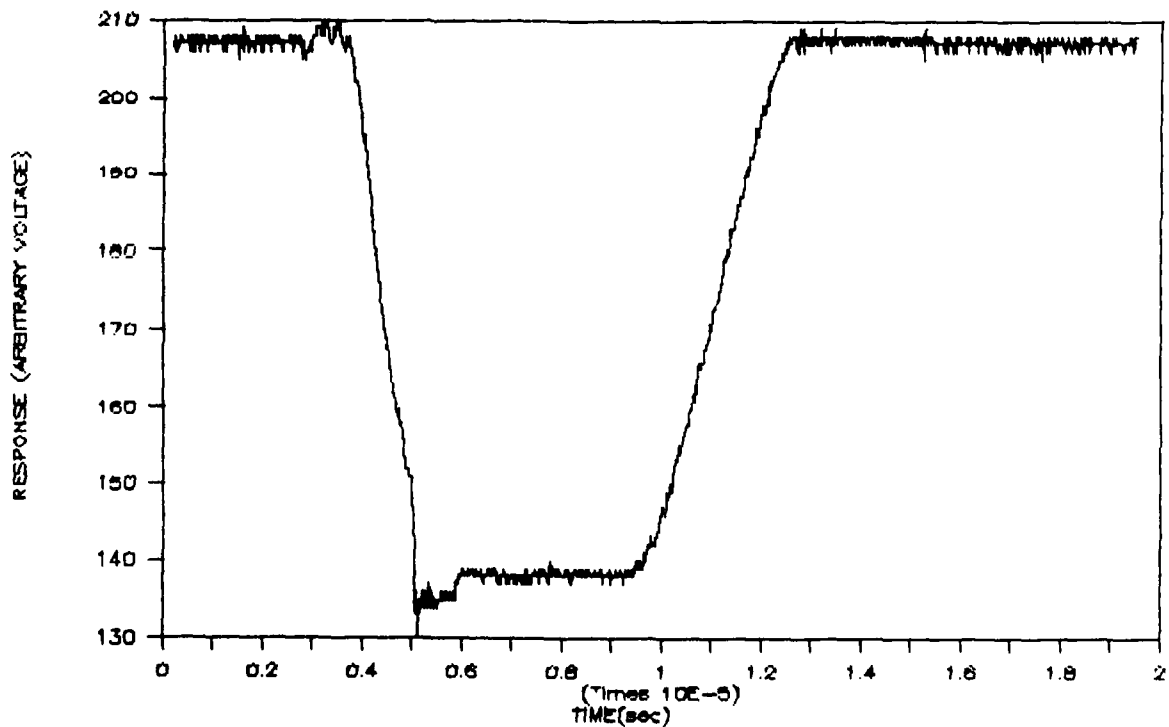
Figure 3 Measured response of TIP122 to 350 ns wide pulse. Note that t_{sr} and t_f are greater than for the 2N4401. The increase in t_{sr} was expected due to large electrical storage time
