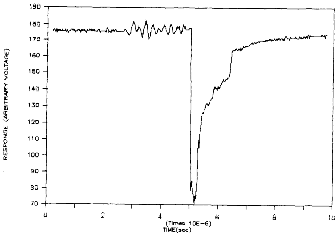
Figure 9 Response of TOS710 MESFET to 2 \mu s wide pulse clearly showing superposition of the two effect discussed in the text
