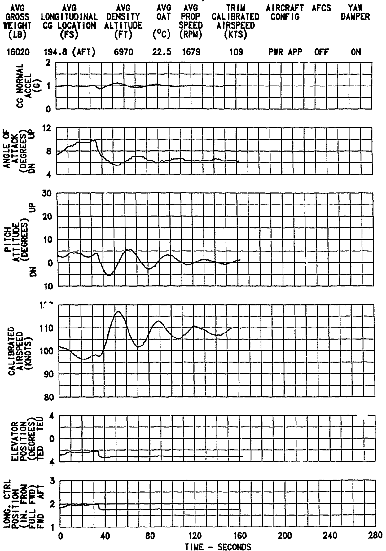
FIGURE E-11 DYNAMIC LONGITUDINAL STABILITY (PHUGOID) RC-12K USA S/N 85-0149
