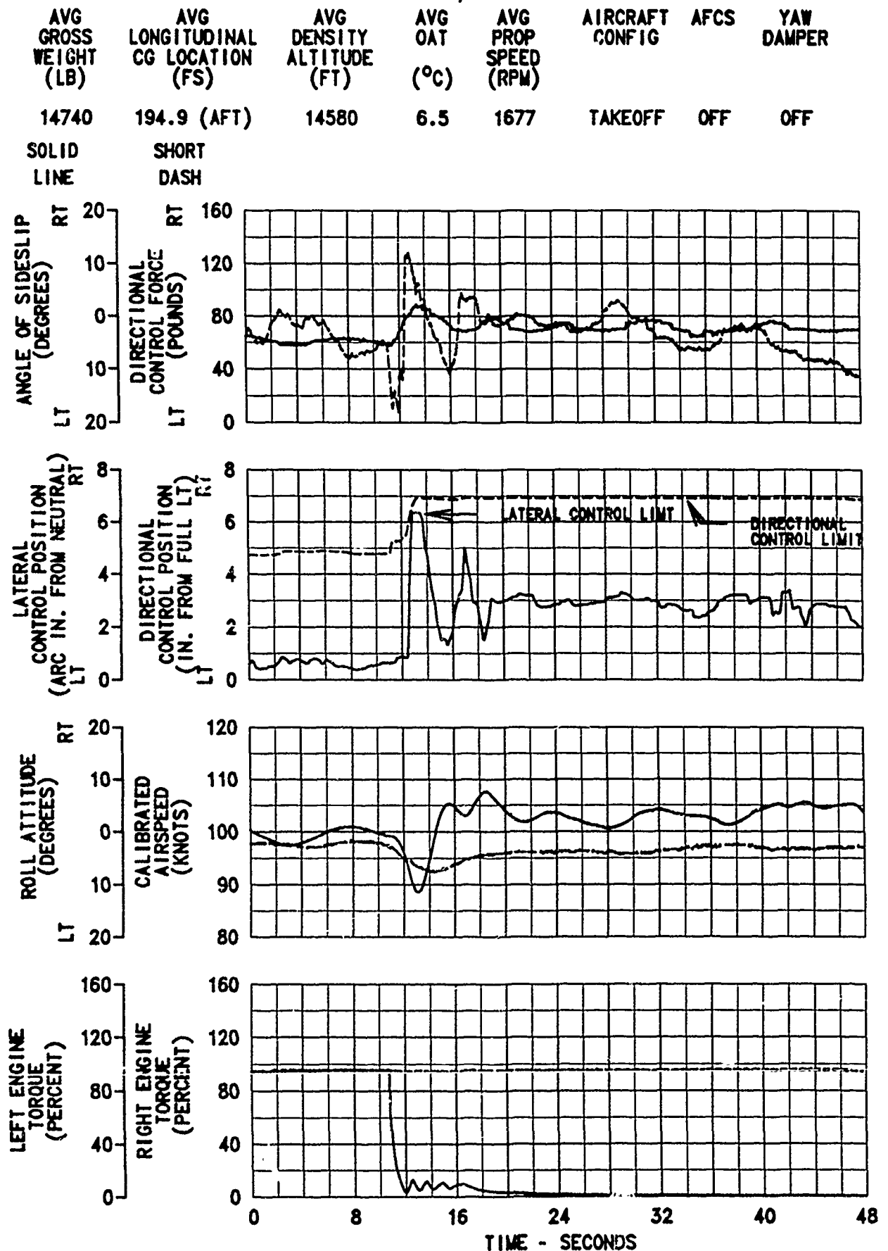
FIGURE E-16 DYNAMIC SINGLE ENGINE MINIMUM CONTROL AIRSPEED (V mc ) RC-12K USA S/N 85-0149
