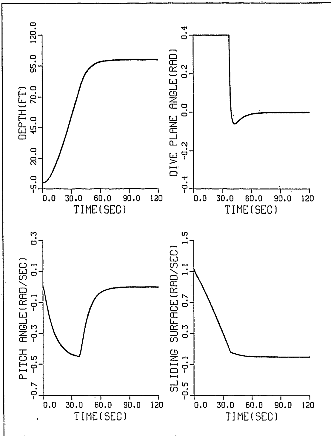
Figure 42. The dynamic response of test 5 AUV (depth command = 100 ft)
