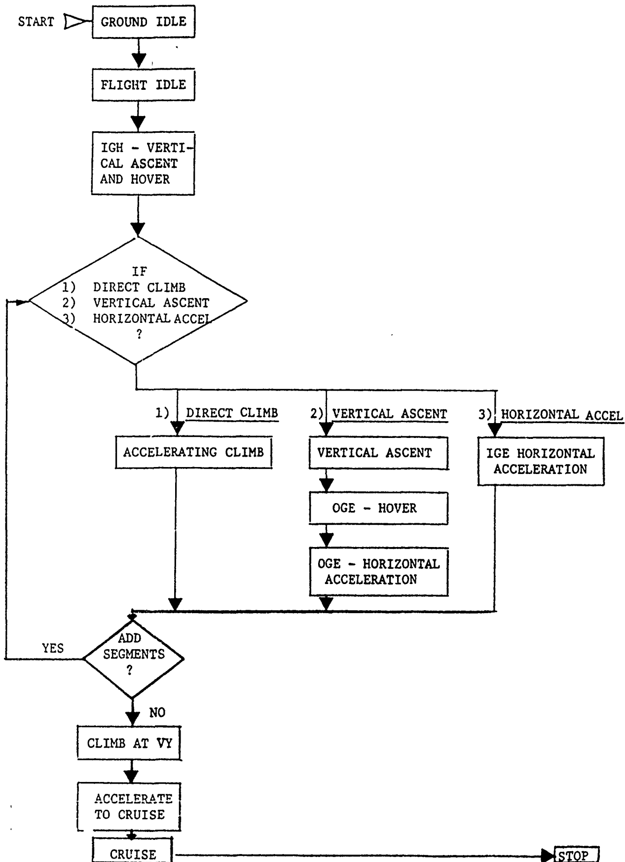
FIGURE 2-4 HNM HELICOPTER DEPARTURE OPERATING MODE INPUT OPTIONS
