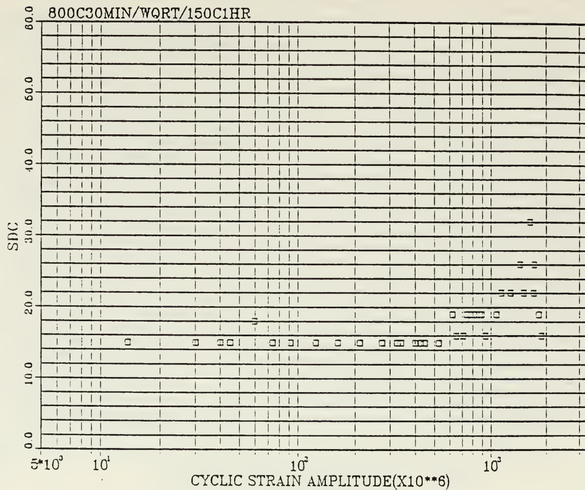
Figure C.6 SDC vs. Strain--Cu-Al-Ni-Mn-Ti 800C30MIN/WQRT/150C1HR/WQRT
