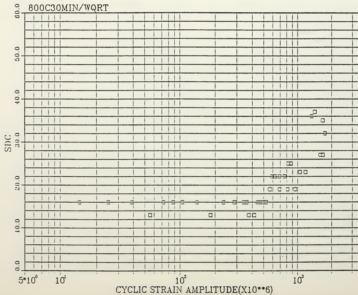
Figure C.5 SDC vs. Strain--Cu-Al-Ni-Mn-Ti 800C30MIN/WQRT
