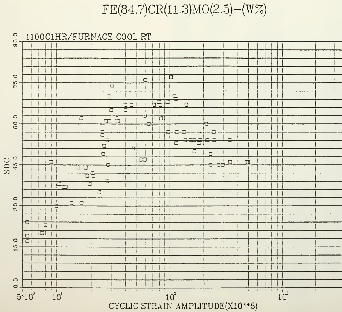
Figure C.1 SDC vs. Strain--FeCrMo
