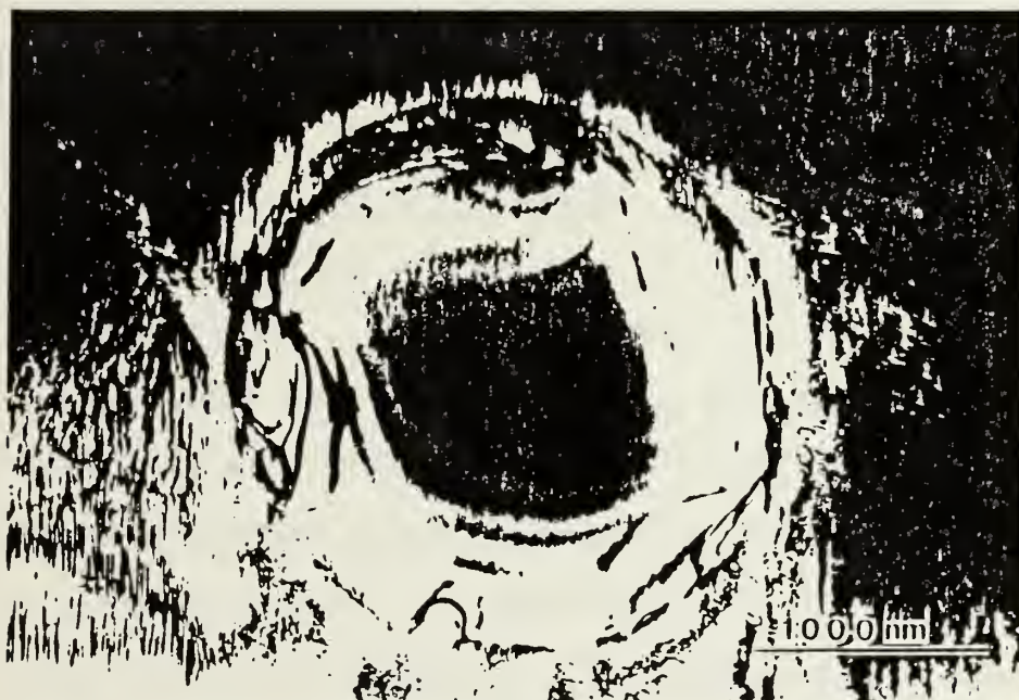
(b) Large X_L Phase Precipitate Particle in Cu-Al-Ni-Mn-Ti
