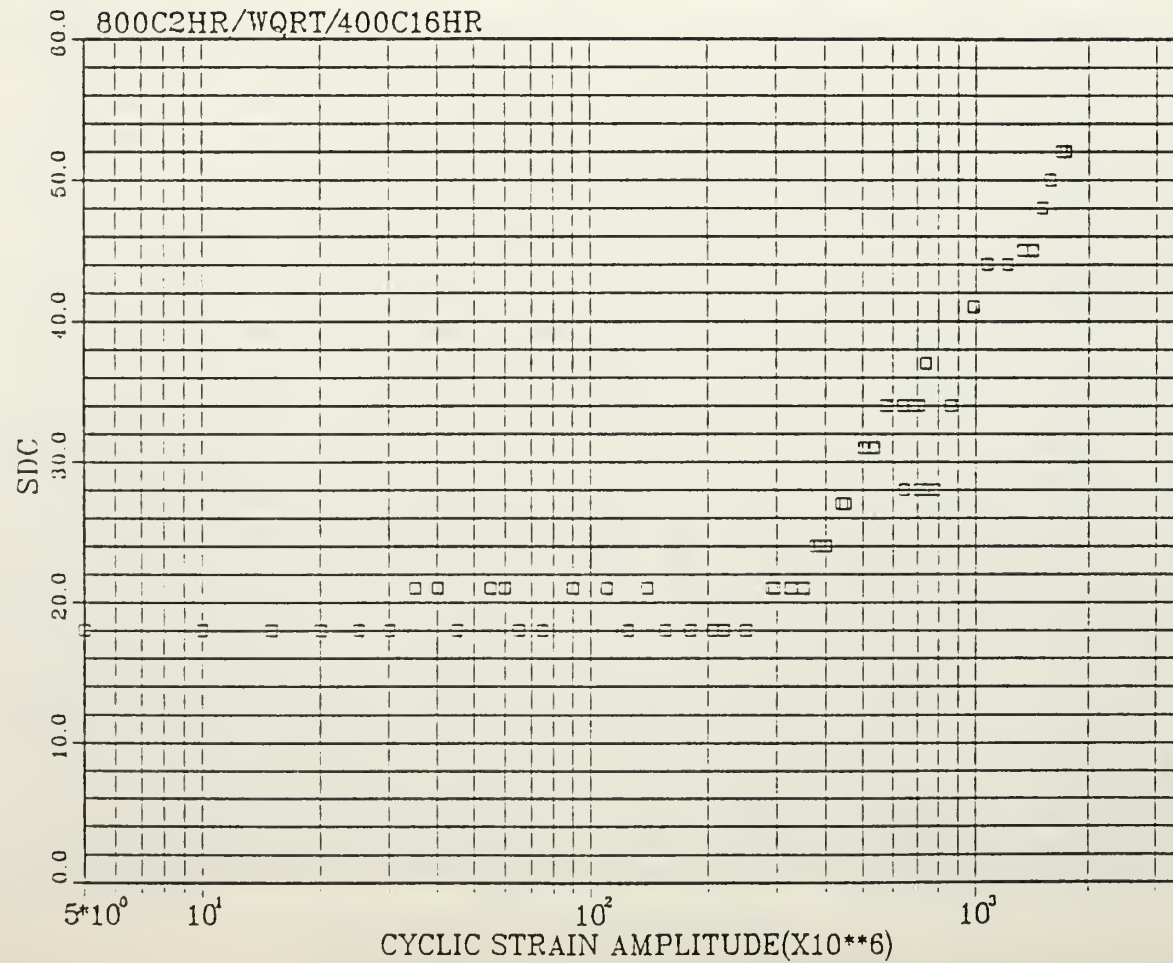
Figure C.3 SDC vs. Strain--INCRAMUTE
