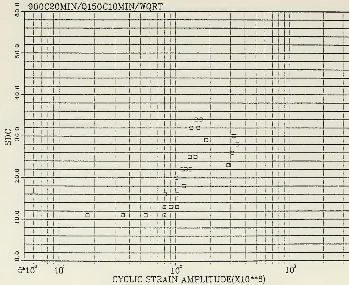
Figure C.4 SDC vs. Strain--CuZnAl
