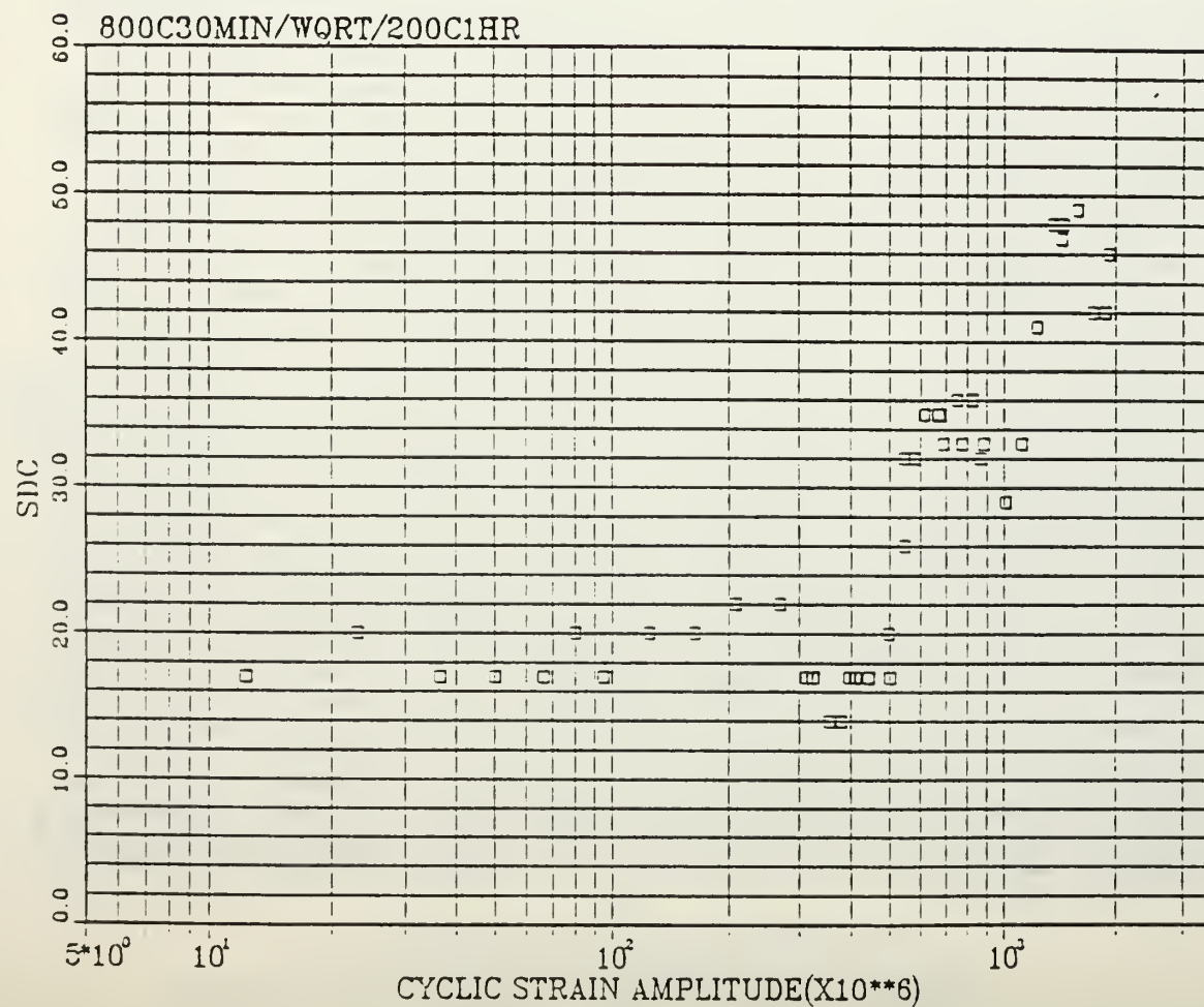
Figure C.7 SDC vs. Strain--Cu-Al-Ni-Mn-Ti 800C30MIN/WQRT/200C1HR/WQRT
