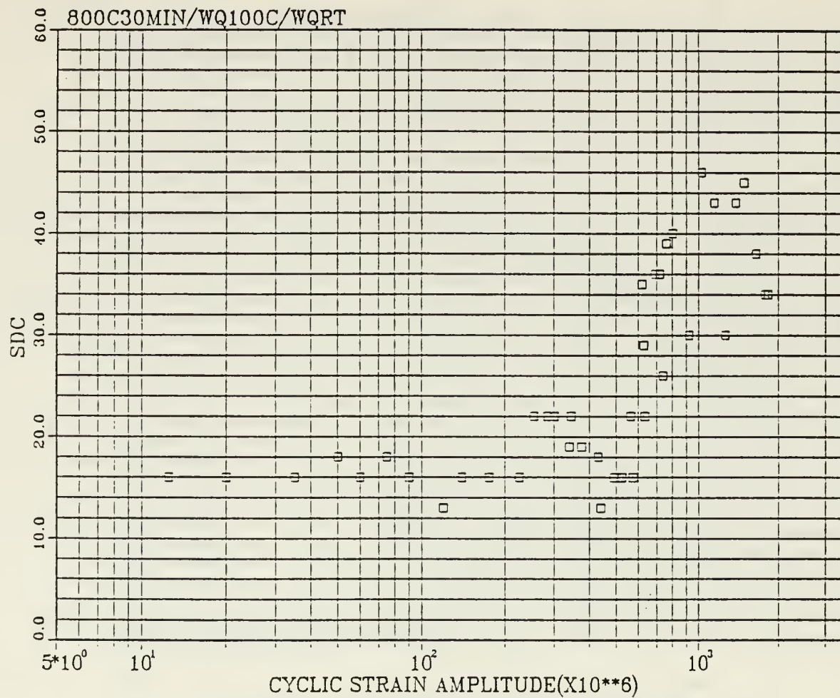
Figure C.8 SDC vs. Strain--Cu-Al-Ni-Mn-Ti 800C30MIN/WQ100C/WQRT
