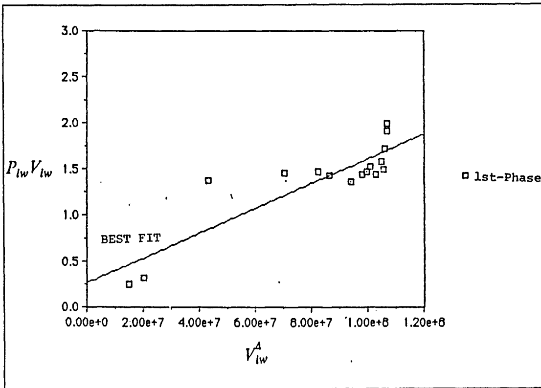
Figure 25. Power Required Linear Regression Plot(Thrust Method)
