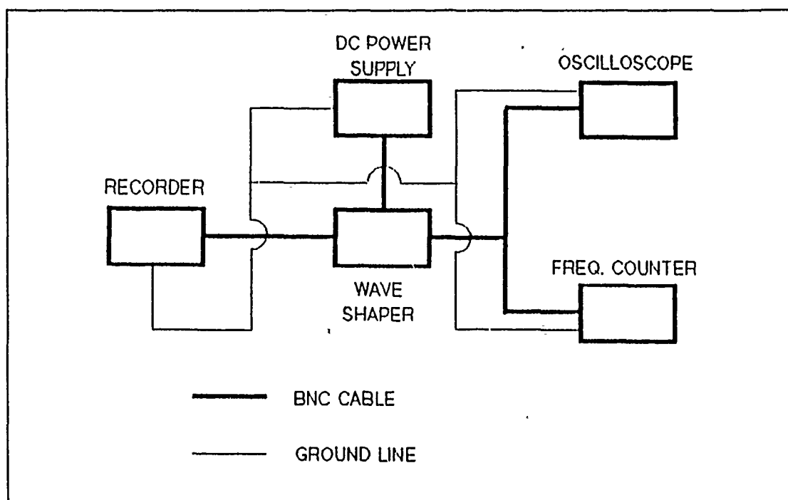
Figure 15. The Network For Signal Conditioning
