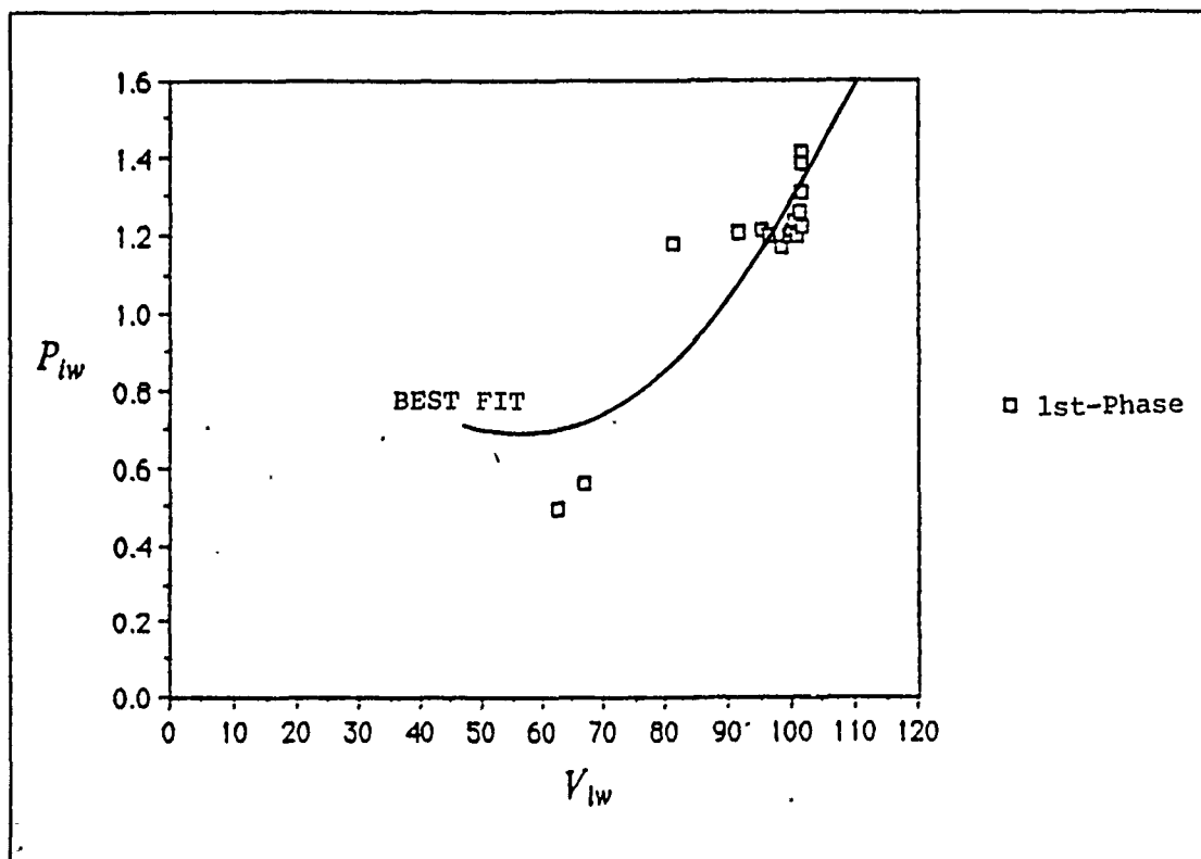
Figure 24. Half-Scale Pioneer Power Required Curve(Thrust Method)
