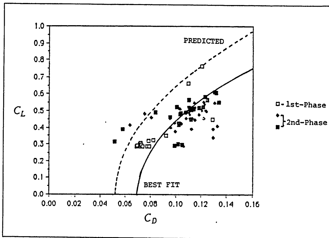
Figure 17. Drag Polar For Original Wing Configuration
