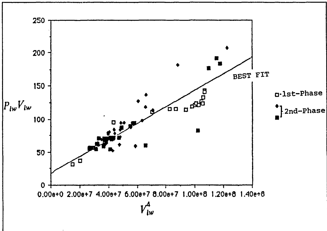
Figure 20. Power Required Linear Regression Plot
