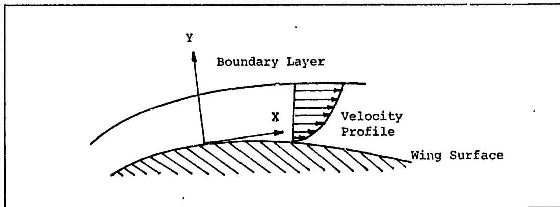
Figure 4. Flow With Friction Over Wing Section
