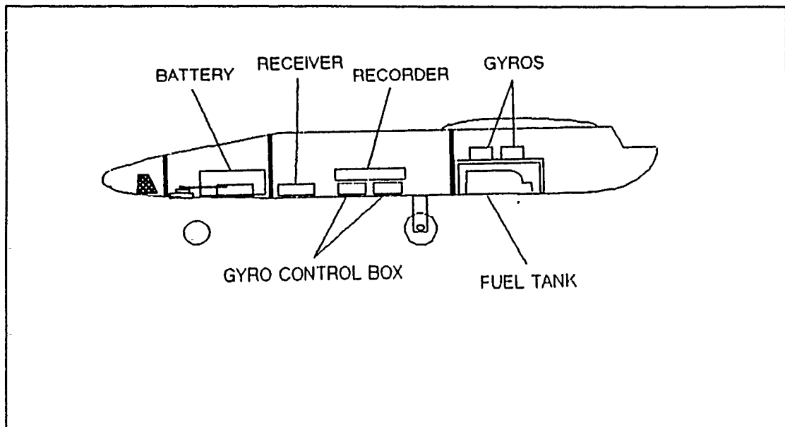
Figure 7. Half-Scale Pioneer Equipment Layout in Body
