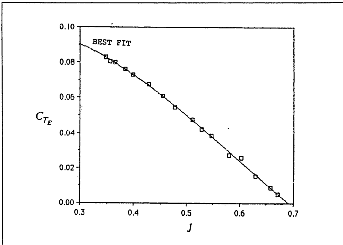
Figure 2. Effective Thrust Coefficient versus Advance Ratio Plot
