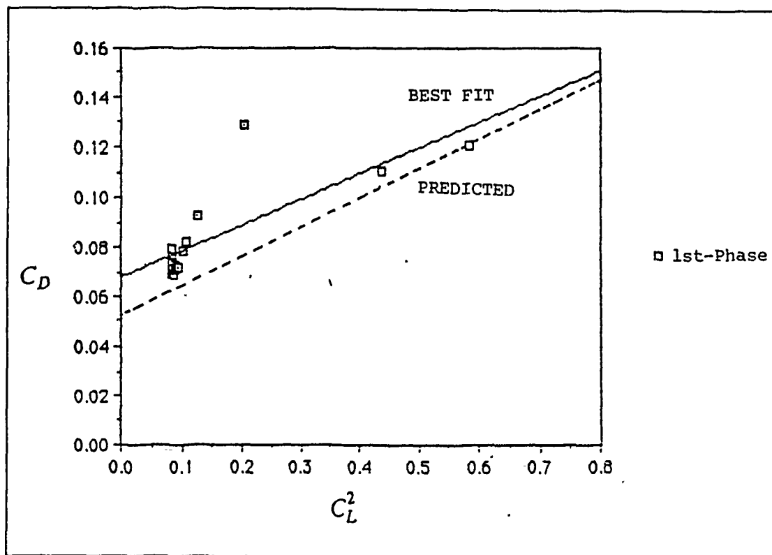
Figure 23. Drag Polar Linear Regression Plot(Thrust Method)
