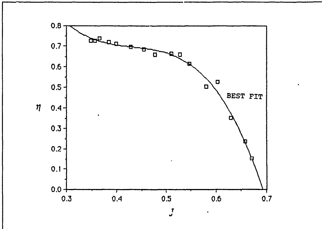
Figure 3. Propeller Efficiency Versus Advance Ratio
