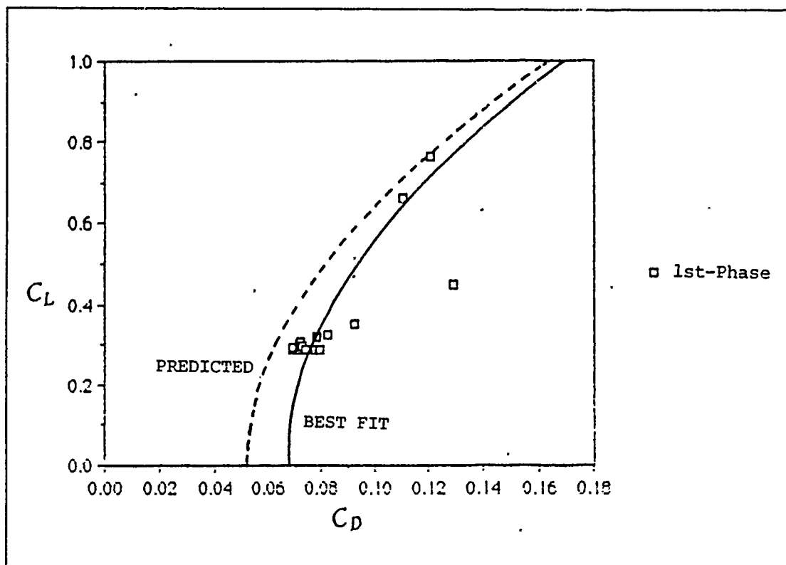
Figure 22. Half-Scale Pioneer Drag Polar Curve(Thrust Method)
