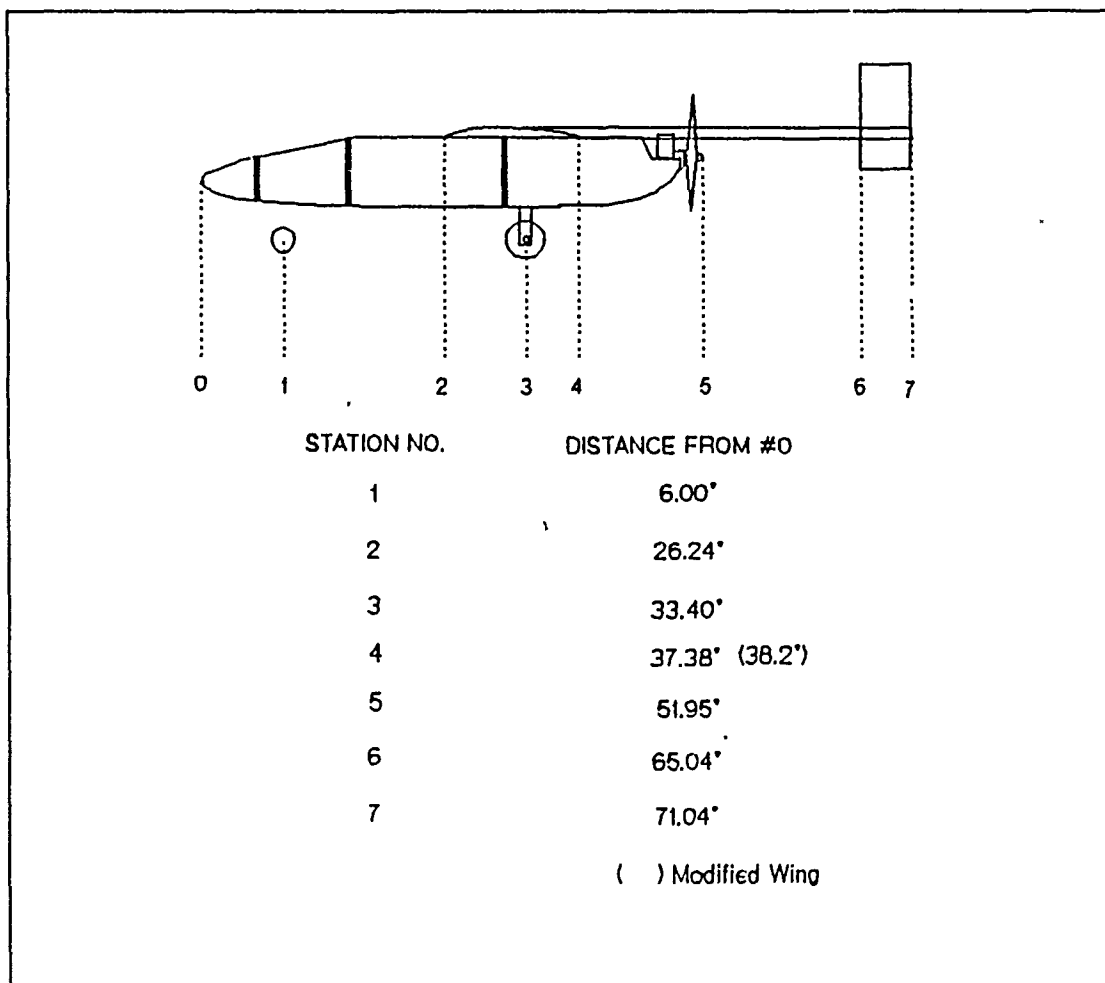
Figure 12. Dimensions for Calculation of C.G.
