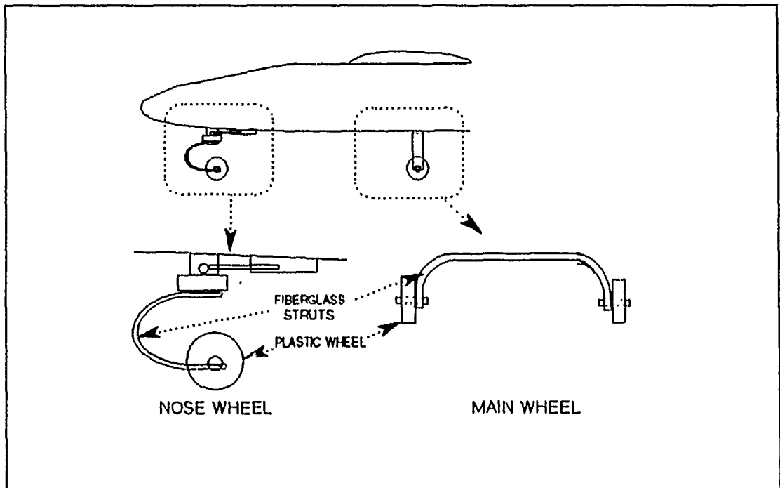
Figure 10. Original Landing Gear System in First Phase
