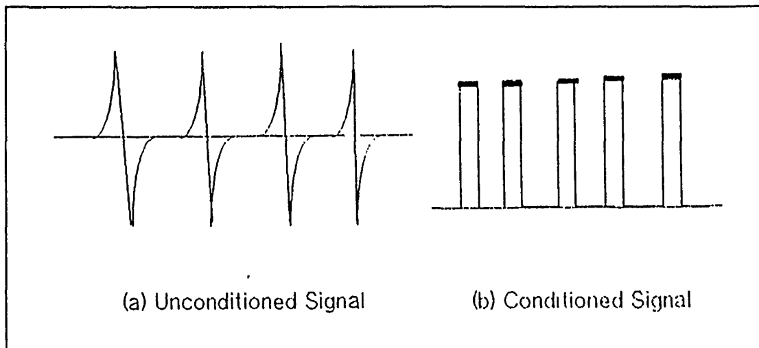
Figure 14. The Results of Signal Conditioning
