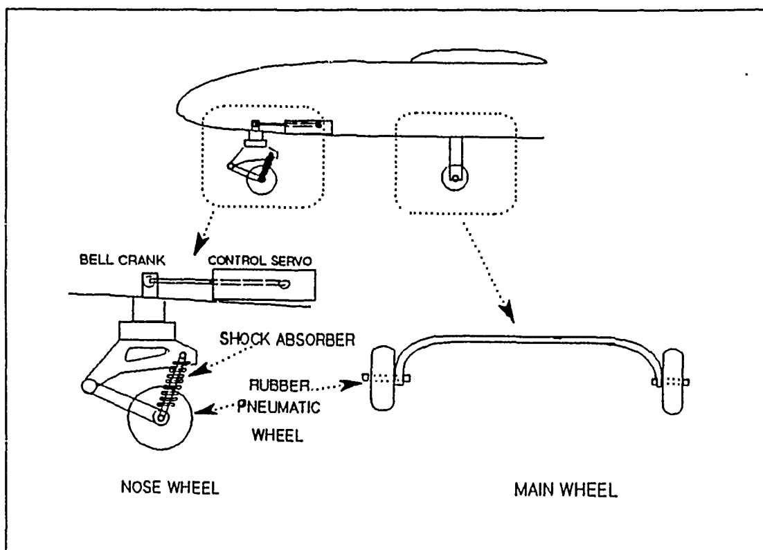
Figure 11. Changed Landing Gear System Configuration
