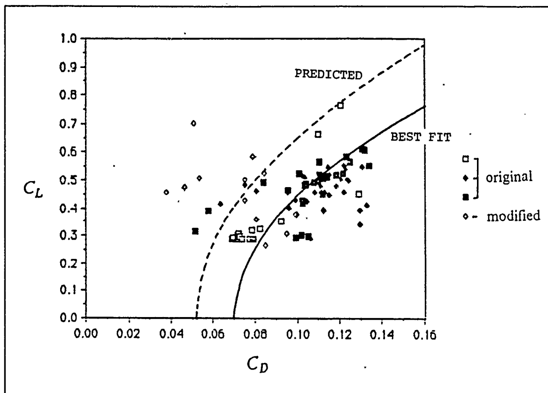
Figure 21. Drag-Polar For Original and Modified Wing Configuration
