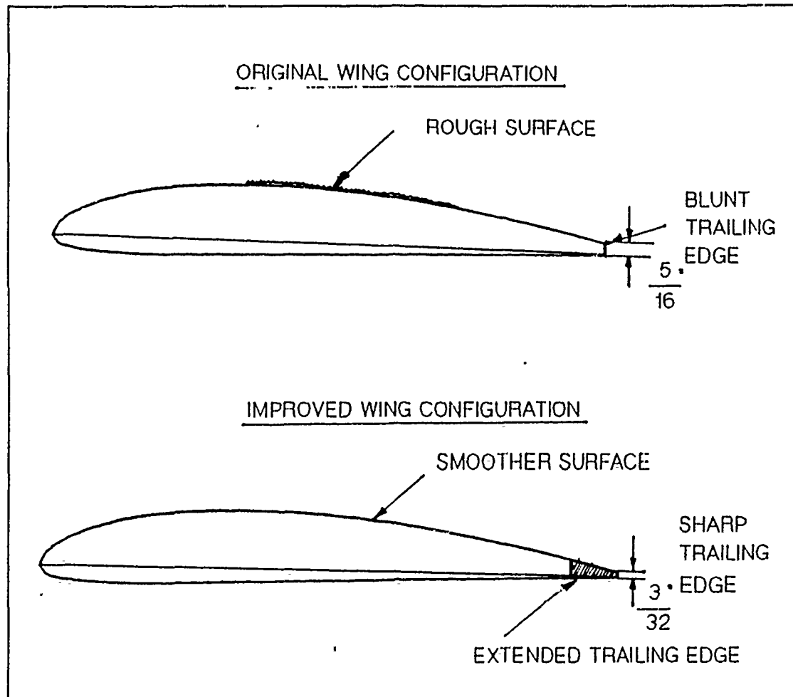
Figure 16. Wing Configuration Changes
