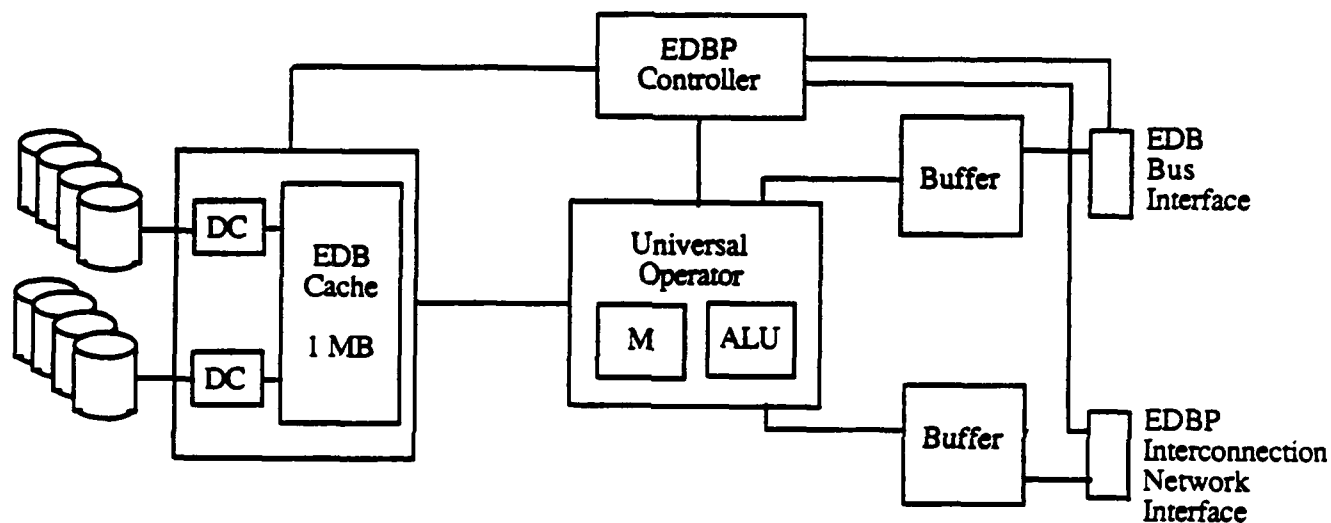
Figure 4. Structure of a Extensional Database Processor
