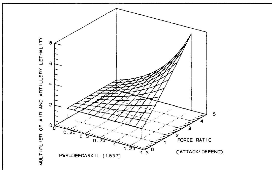
Figure 15. PWRCOFCASKIL Determines How Force Ratio (Representing Relative Target Density) Increases the Weaker Force's Air and Artillery Lethality.
