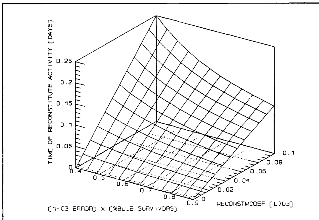
Figure 26. RECONSTMCOEF Determines How C3 Error and the Fraction of Blue Survivors Combine to Determine Time to Reconstitute Blue Forces.
