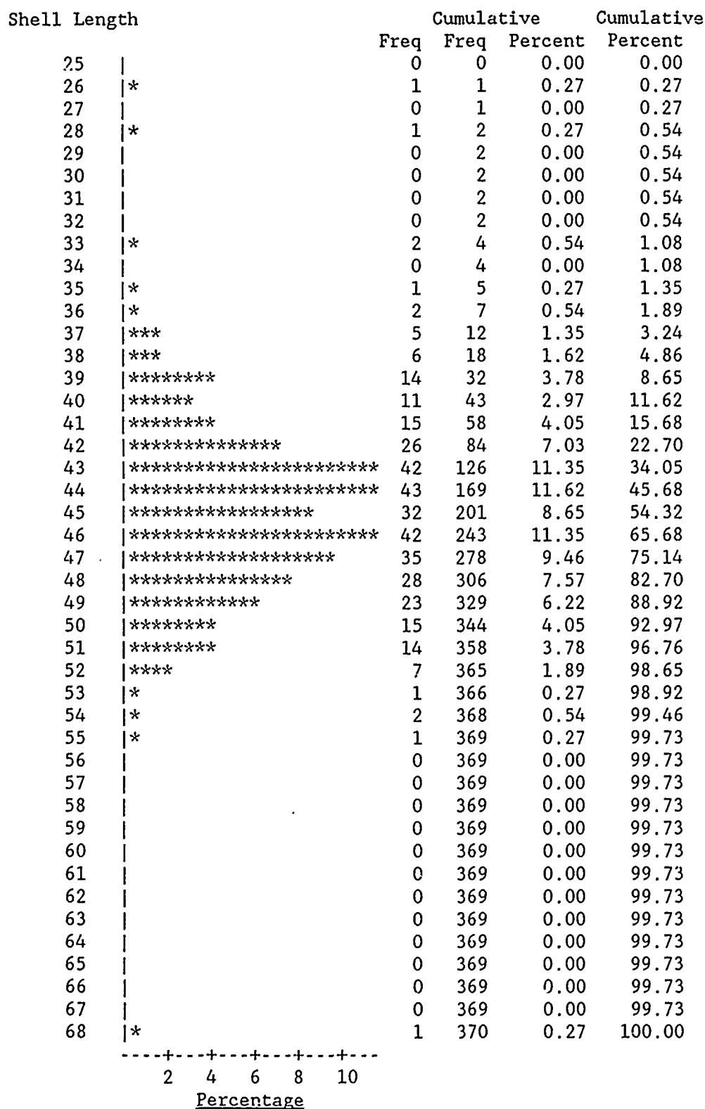
Figure E4. Shell length frequency histogram of Anodonta imbecillis in the upper Mississippi River, RM 450.4 (Pool 17), 25 July 1988
