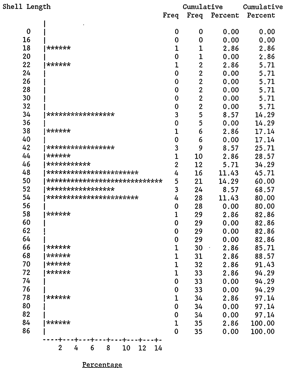
Figure E12. Shell length frequency histogram of Quadrula quadrula in the upper Mississippi River, RM 433.3 (Pool 18), 23 July 1988
