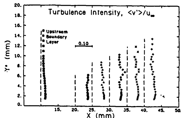
Fig. 11 Vertical turbulence intensity profiles for the 16-deg compression corner flowfield.
