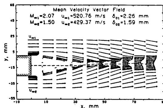
Fig. 6 Mean velocity vector field
