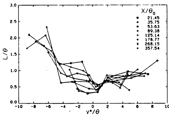
Fig. 12 Mixing length profiles for the ramp flowfield, L = |\langle u'v' \rangle|^{1/2} / (dU/dy) .
