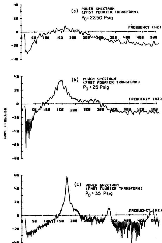
Fig. 5 Power spectra of base pressure oscillations for: a) L = 101 mm, P_0 = 22.5 psig; b) L = 101 mm, P_0 = 25 psig; and c) L = 101 mm, P_0 = 35 psig.
