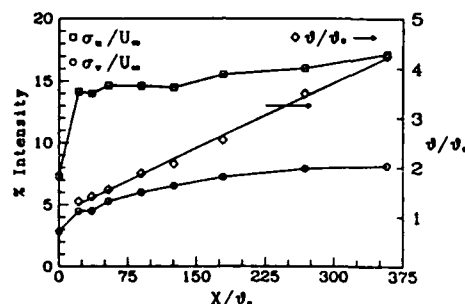
Fig. 10 Local maximum turbulence intensities and momentum thicknesses for the ramp flowfield mixing layer. The linear least-squares fit to the momentum thickness data, used to estimate the entrainment rate, is shown.
