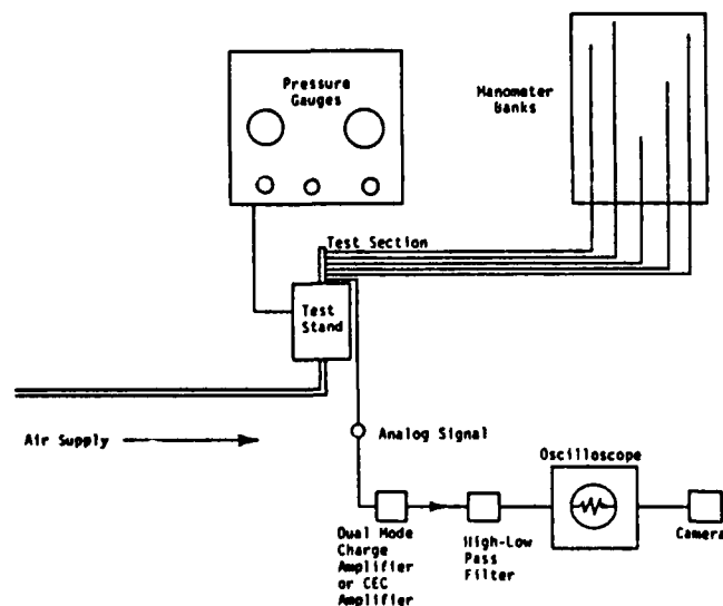
Fig. 11 Data acquisition flow diagram for channel pressure history experiments.
