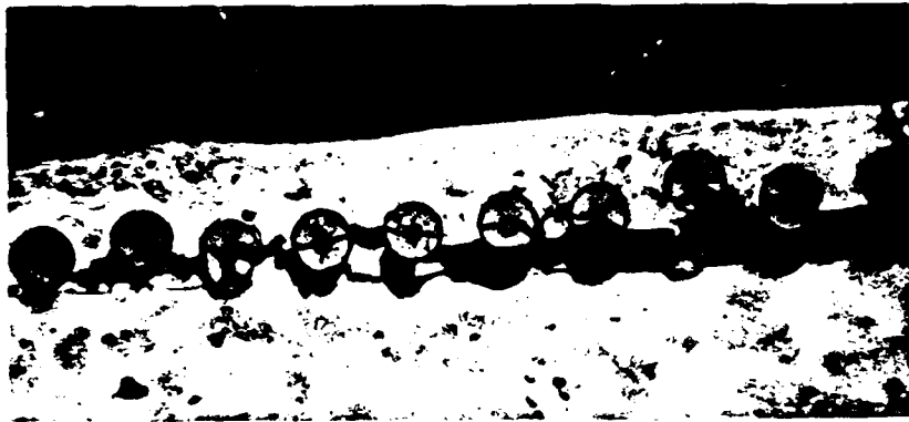
Figure 3.5.4.2.3 Ply separation during machining of 4" diameter trial RFl122 for Ti_3Al/SCS-6 MMC.
