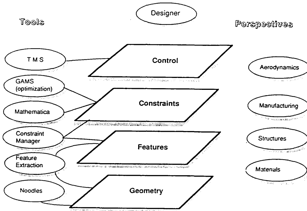
Figure 1: Flow of control in Design Fusion
