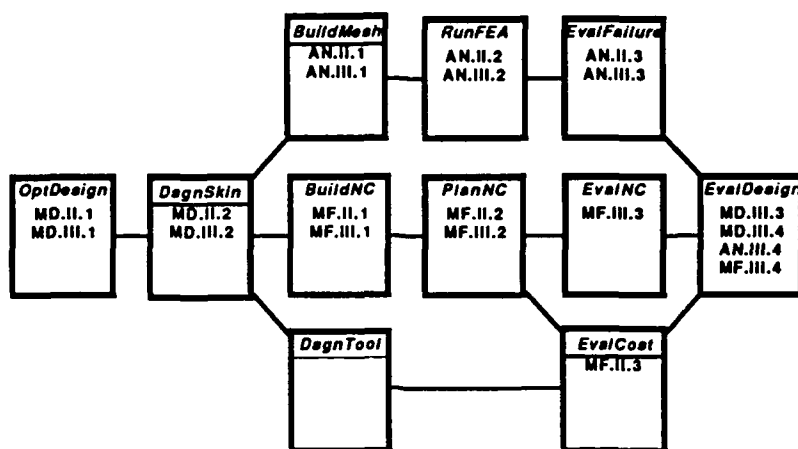
Activity diagram (fragment)
