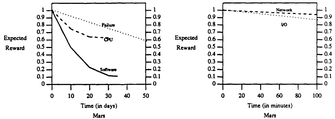
Expected Reward Rate for Mars. Figure 4.2
