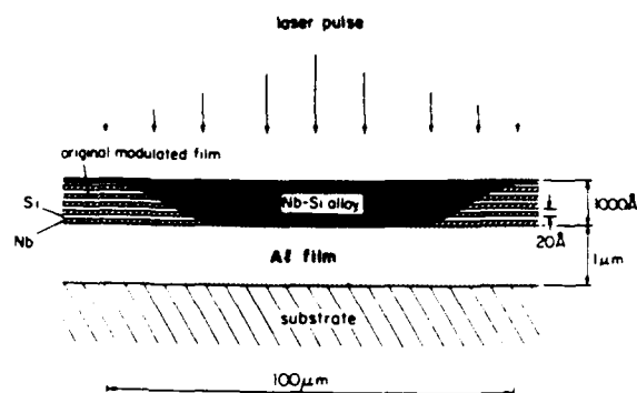
Fig. 2. Schematic diagram (on a variable scale) of a multilayer film after irradiation with a laser pulse with a gaussian intensity profile.
