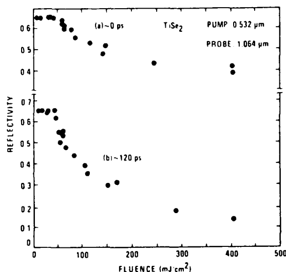
Figure 3. Reflectivity of 1T\text{-TiSe}_2 at 1.064 \mu\text{m} as a function of 0.532 \mu\text{m} pump fluence at the delay (a) - 0 ps and (b) - 120 ps.
