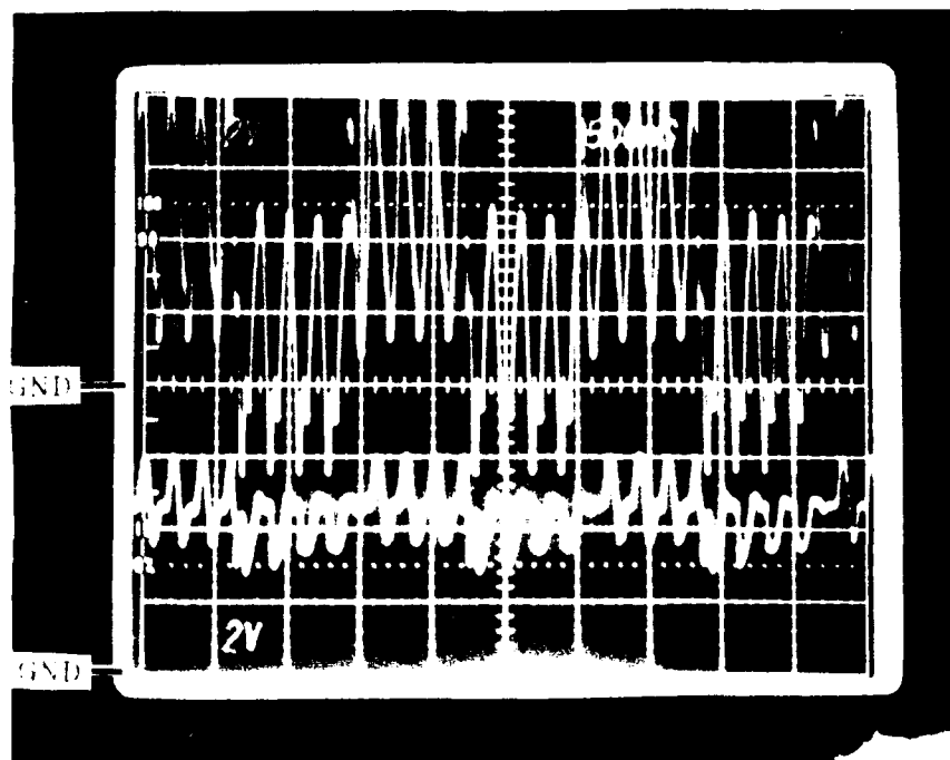
Figure 9.3.1.2 - CD4013B Oscilloscope Photograph, No RF Top trace = Data input Bottom trace = Q output
