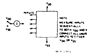
Fig. 10 - Input current test circuit
