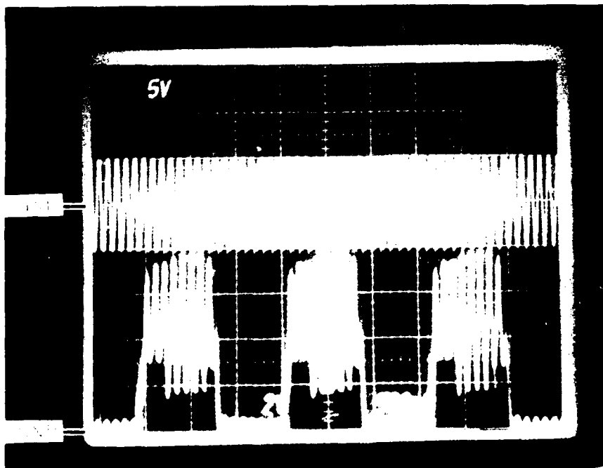
Figure 8.3.9 - CD4013B RF Upset Oscilloscope Photograph RF Interference on Vdd Top trace = 10 MHz RF Bottom trace = Q output
