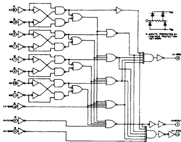
Fig. 4 - Logic diagram
