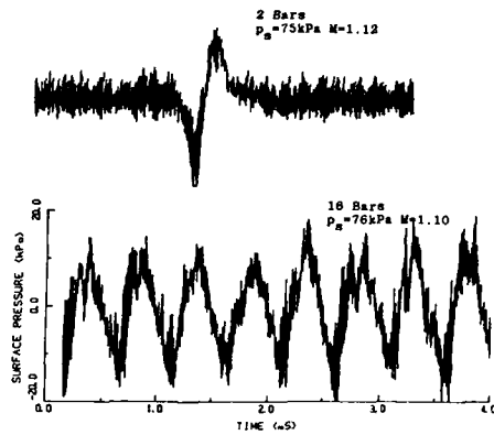
Fig. 3 Raw time resolved surface pressure measurements presented for the 2 bar and 16 bar cases. M_{brl} = 0.75 . Suction surface MP P16, \lambda/ca\lambda = 0.39 .
