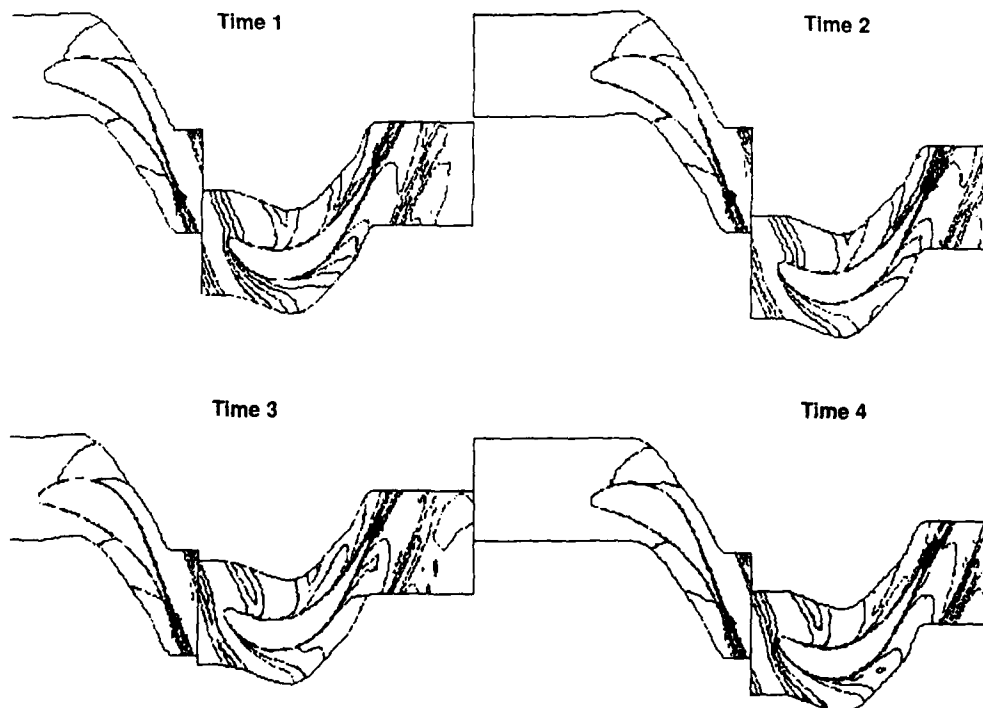
Figure 5: Entropy contours showing stator-wake/rotor relative location at four equally spaced times within one ROTOR1 cycle.
