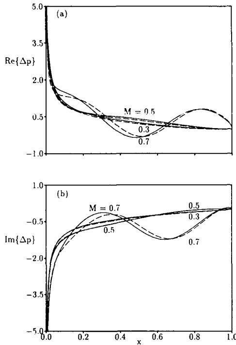
Figure 4: Effect of Mach number on the unsteady pressure-difference response of a flat-plate cascade with \Omega = \Theta = 45 deg and G = 1 subjected to an incident vortical gust with v_g = (1, 0) , \omega = 5 and \sigma = -2\pi : (a) in-phase component (real part) of \Delta p , (b) out-of-phase component (imaginary part); --- Smith analysis [4], — present analysis.
