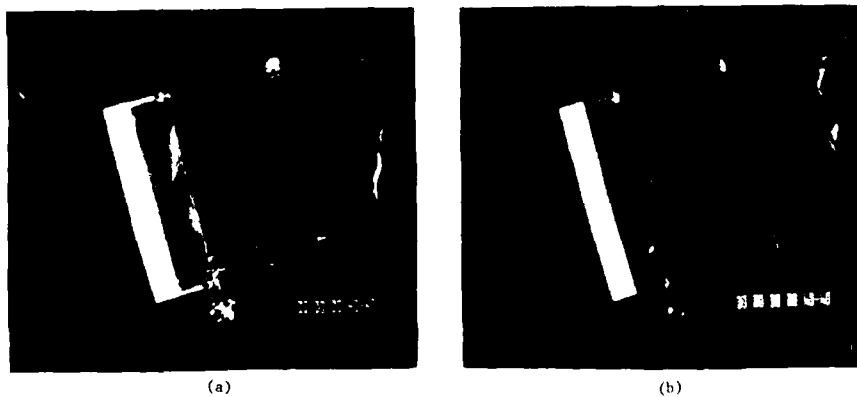
Figure 5 Smoke wire (a) and Hot Wire (b) Visualisation of Flow in the model at 15° Incidence (Hucknall Facility)
