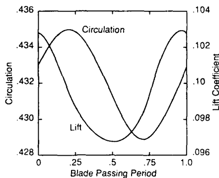
Fig. 5: Time variation of rotor blade circulation and lift as a function of blade passing period (time required to traverse one stator pitch)
