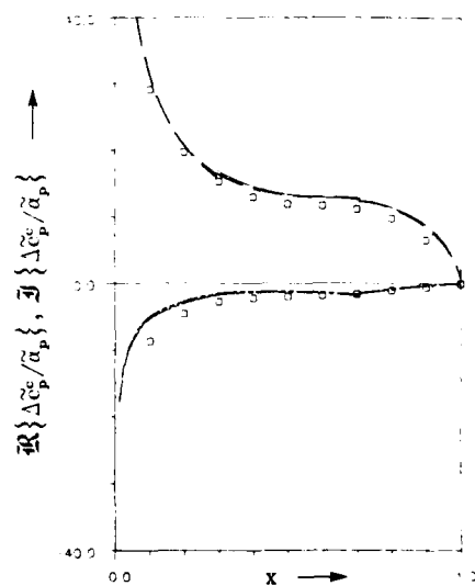
Fig. 11 Real and imaginary part of the unsteady pressure difference at the surfaces of flat plate and double circular airfoils in cascades with l/d = 0.707 , M_\infty = 0.9 , \epsilon_d = 0.0035 , \epsilon_s = 0.002 . \alpha is chosen such that there is no flow around the leading edge, k = 0.092 , \sigma = 180^\circ , \hat{\alpha}_p = 0.0016 .
