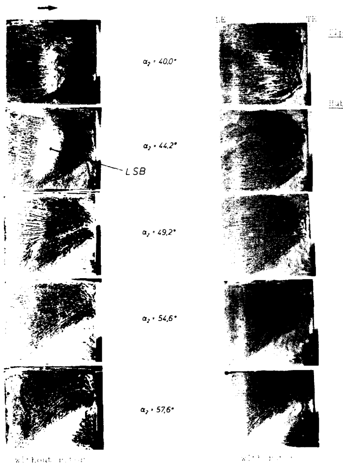
Fig. 1. Flow visualization in the subsonic flow.
