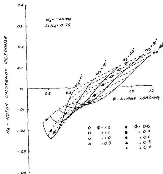
Figure 7 - Rotor Unsteady Response \alpha_2 = -20 deg and s_R/c_R = 0.75
