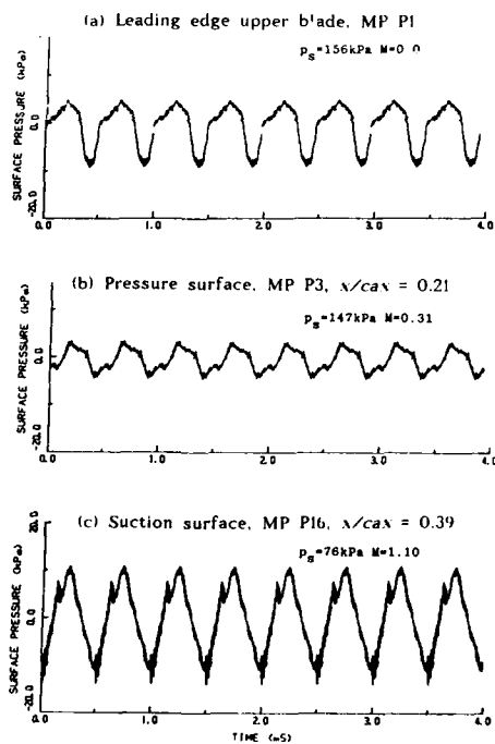
Fig. 4 Ensemble averaged time resolved surface pressure measurements for 16 bar, M_{brl} = 0.75 .
