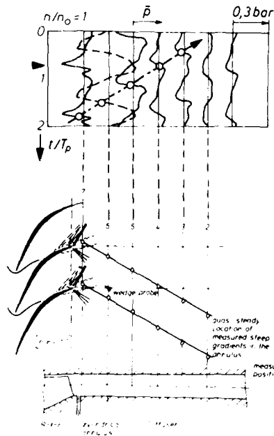
Fig. 13b: Location of trailing-edge shocks downstream of the rotor
