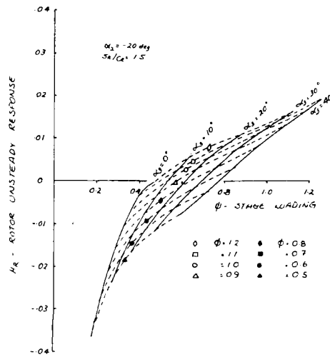
Figure 5 - Rotor Unsteady Response \alpha_2 = -20 \text{ deg} and s_h/C_h = 1.5
