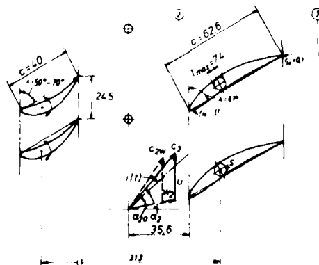
Fig. 2: Cascade geometry at mid-span (units in mm)
