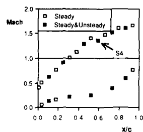
Fig 7a: Cascade II: Steady state flow conditions ( \beta_1 = -13^\circ , M_{25} = 1.43 ). Unsteady pressure transducer locations are marked by closed symbols.
