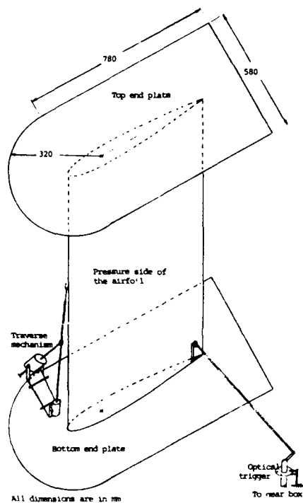
Figure 1 : Experimental set-up
