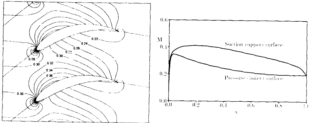
Figure 7: Mach number contours and blade surface Mach number distributions for a steady flow with M_{\infty} = 0.3 and \Omega_{\infty} \approx 40 deg through the EGV cascade ( \theta = 15 deg, G \approx 0.6 , H_f = 0.12 and H_c = 0.13 ).
