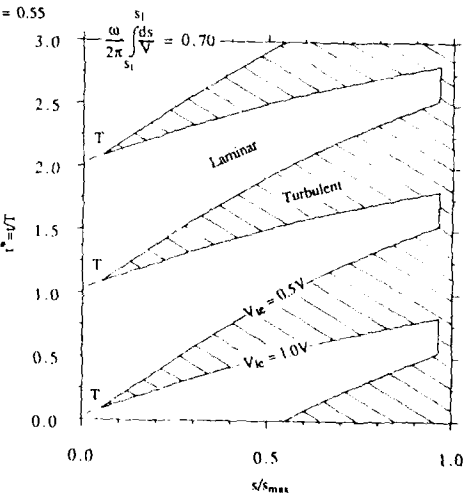
Fig. 11 Distance-time diagram of boundary layer states showing effect of non-uniform velocity distribution for Speidel's Kanal II aerofoil
