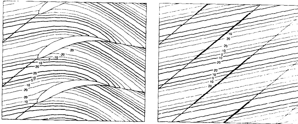
Figure 8: Contours of the real part of the unsteady vorticity for the EGV and the corresponding flat-plate ( M = 0.3 , \Omega = \theta \approx 40 deg, G = 0.6 ) cascades subjected to an incident vortical gust with v_g = (1, 0) , \omega = 5 and \sigma = -2\pi .
