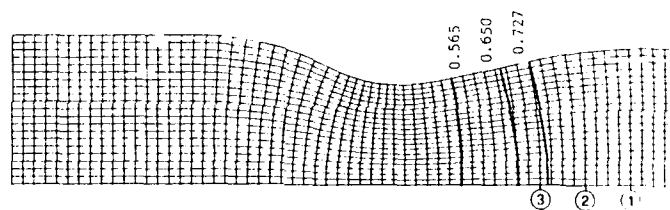
Fig. 5 - Transonic nozzle
